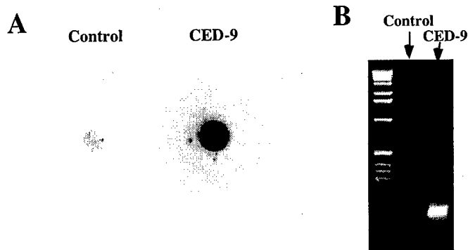
Figure 3. Optimizing protein-RNA binding conditions in the first round of SELEX. A. Filter-binding assay to isolate CED-9/RNA complexes (RNAs were labeled with 32 P). B. Amplification selected RNAs by RT-PCR,
