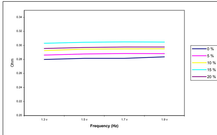
Figure 55. Resistance of Uninsulated Copper Yarn Woven into Fabric at different Applied Voltages and Tensile Strains
