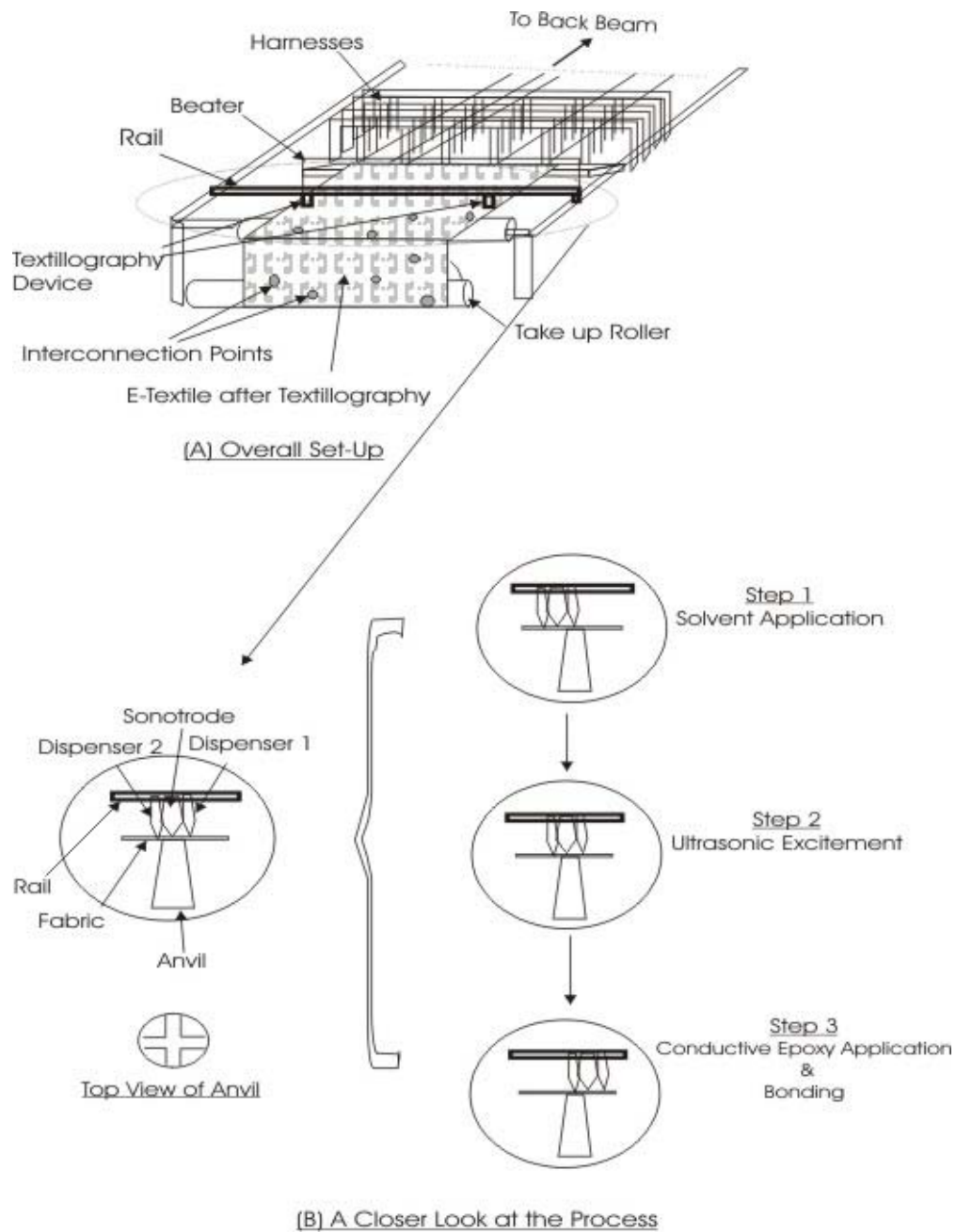
Figure 69. Schematic of On-Loom Textillography
