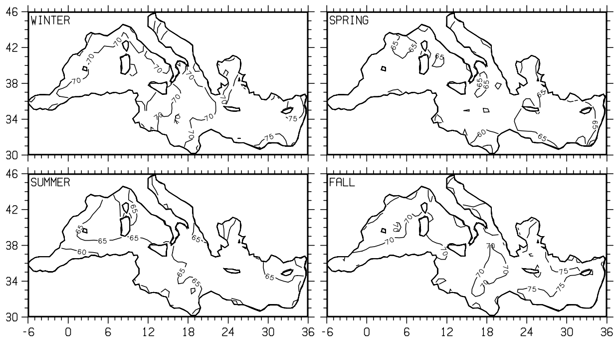
Fig. A5 — Seasonally averaged climatological longwave radiation (contour interval is 5 W/m 2 )
