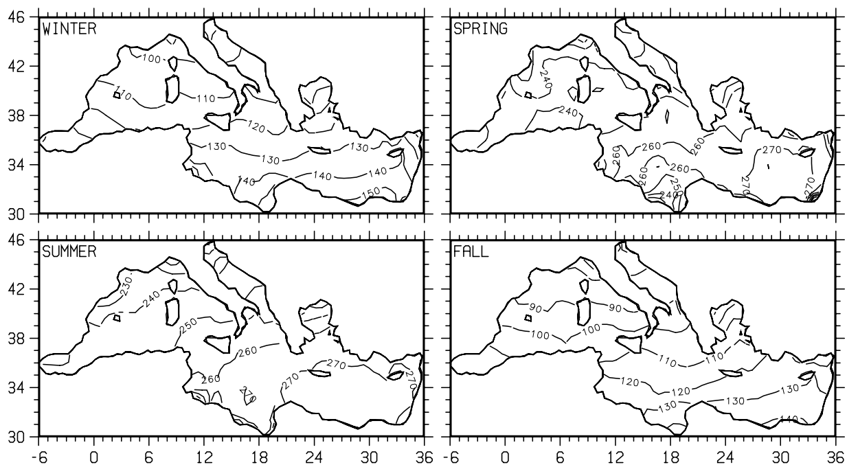
Fig. A4 — Seasonally averaged climatological solar radiation (5 % albedo applied, contour interval is 10 W/m 2 )
