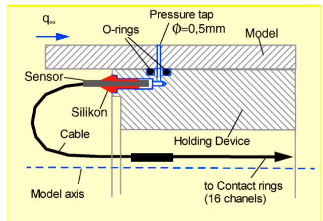
Figure 3. Connection from pressure tap to Kulite sensor in the spinning model
