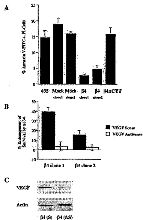
Figure 1. The \alpha 6\beta 4 -mediated survival of breast carcinoma cells is VEGF dependent. (A) Parental, mock (clone 1, 6D2; clone 2, 6D7), \beta 4\Delta CT-expressing (cytoplasmic tail deletion mutant), and \beta 4 integrin-expressing (clone 1, 3A7; clone 2, 5B3) MDA-MB-435 subclones were maintained in low serum (0.5% FBS) medium for 24 h. To assess the level of apoptosis, these cells were stained with annexin V-FITC and propidium iodide (PI), and analyzed on a Becton Dickinson flow cytometer using CellQuest software. The percentage of annexin-positive, PI-negative cells ( \pm SD) is indicated. Results were obtained from three independent experiments. Apoptosis was minimal in the presence of 10% FBS (unpublished data). (B) Mock-transfected clone 6D7 and \beta 4 integrin-expressing (clone 1, 3A7; clone 2, 5B3) MDA-MB-435 subclones were transiently transfected with VEGF sense or antisense oligonucleotides and maintained in low serum (0.5% FBS) medium. After 24 h, the level of apoptosis in these cells was assessed as described above. The data are presented as the mean difference ( \pm SD) in annexin positivity between mock-transfected and \alpha 6\beta 4 -expressing MDA-MB-435 cells. Similar results were observed in two separate experiments. (C) The relative amount of VEGF protein in extracts obtained from the MDA-MB-435/ \beta 4 cells transfected with either the VEGF sense (S) or antisense (AS) oligonucleotide was determined by immunoblotting using a polyclonal anti-VEGF immune serum.
