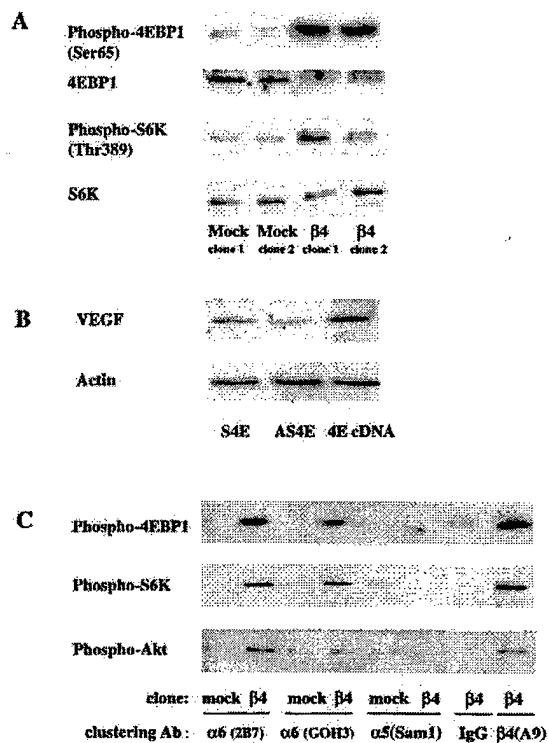
Figure 4. The \alpha 6 \beta 4 integrin stimulates the phosphorylation of Akt, 4E-BP1, and p70 S6K . (A) MDA-MB-435 parental cells, mock transfectants, and \beta 4 transfectants were maintained in medium containing low serum (0.5% FBS) for 24 h. The phosphorylation status of 4E-BP1 on Ser 65 and S6K on Thr 389 was assessed in extracts from these cells using phosphospecific antibodies as described in the Materials and Methods. In addition, the total amount of 4E-BP1 and p70 S6K in these extracts was assessed by immunoblotting. (B) The MDA-MB-435/ \beta 4 cells were transiently transfected with either an eIF-4E sense (S) or antisense (AS) oligonucleotide, or a full-length eIF-4E cDNA (4E). Extracts of these cells containing equivalent amounts of protein were analyzed for their relative expression of VEGF and actin by immunoblotting. (C) MDA-MB-435 mock (clone 6D7) and \beta 4 (clone 3A7) transfectants were maintained in low serum (0.5% FBS) medium for 24 h. These cells were detached with trypsin and incubated with integrin-specific antibodies ( \alpha 6 integrin, 2B7; \alpha 6 integrin, GOH3; \alpha 5 integrin, Sam1; \beta 4 integrin, A9) or IgG for 30 min as described in the legend to Fig. 2. The phosphorylation status of 4E-BP1 (Ser 65), S6K (Thr 389), and Akt (Ser 473) was assessed in extracts from these cells using phosphospecific antibodies. Similar results were observed in four independent experiments.
