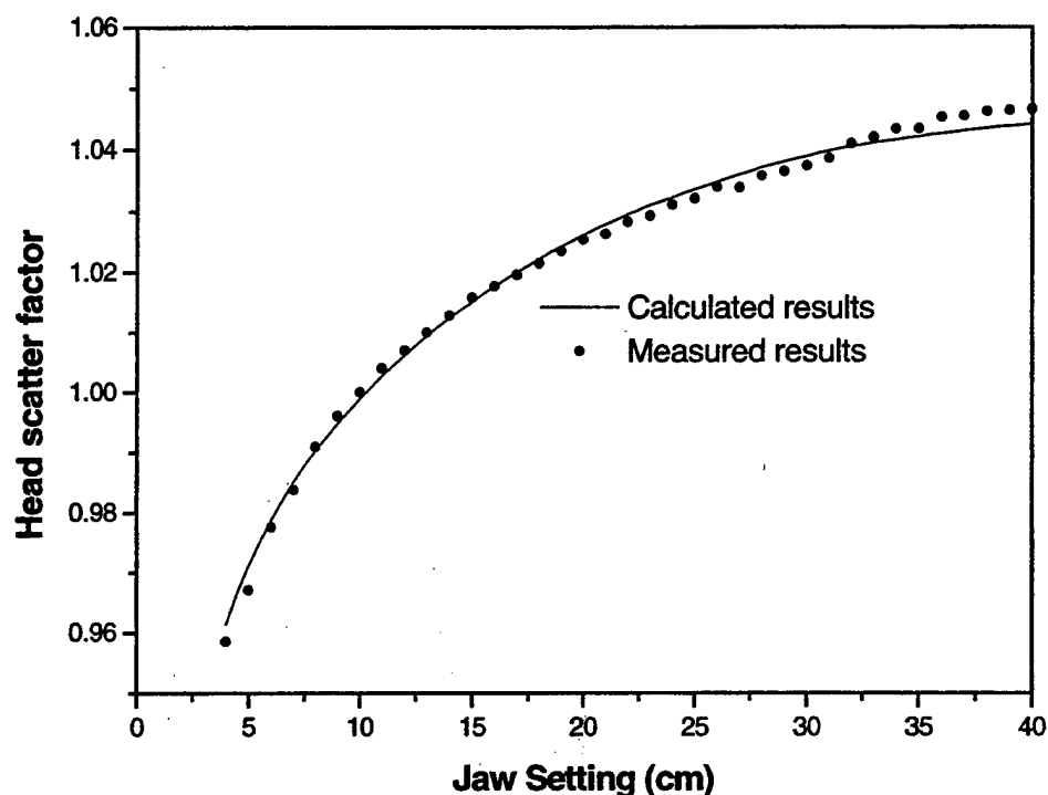
Fig. 4. The measured and calculated head scatter factors for square field size from 4 cm to 40 cm at isocenter for 15 MV photon beam. All the data are normalized to the value of a 10 \times 10 cm 2 field at SAD. The line and solid dots represent the calculated and measured data, respectively.
