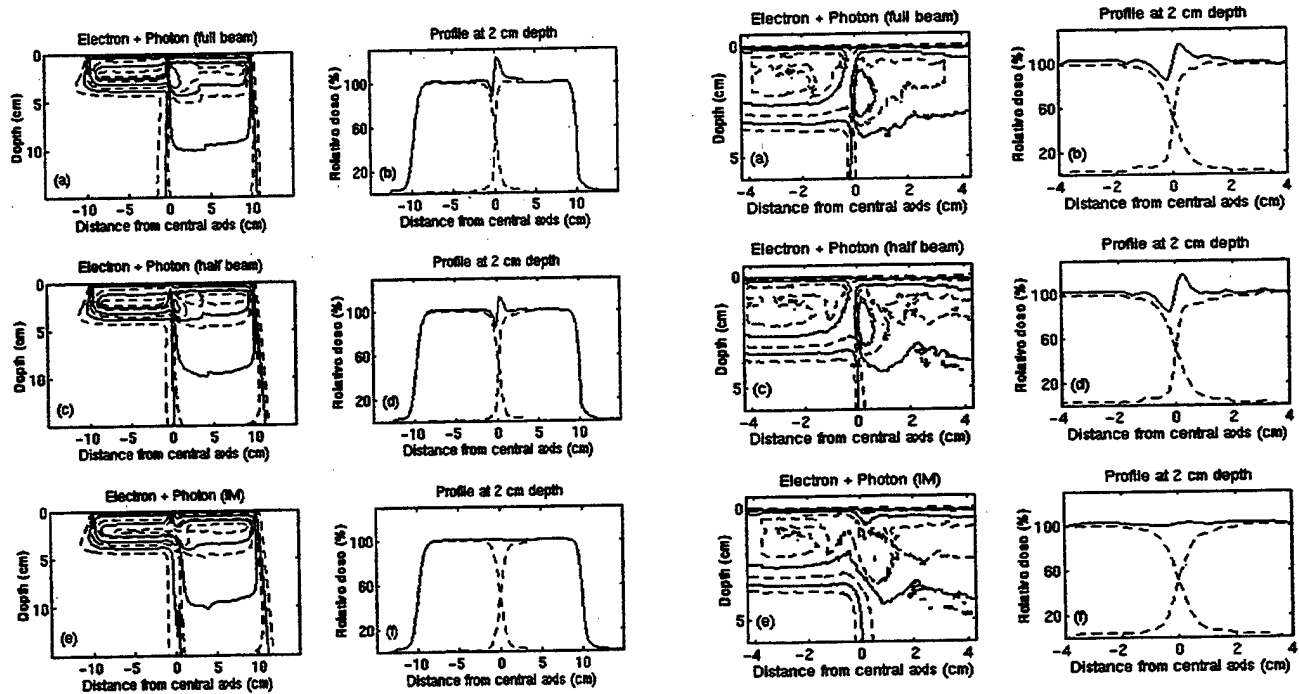
Fig. 1 Matching of electron-photon fields. The left two columns are theoretical calculations and the right two columns are film measurements. A divergent (full-beam), non-divergent (half beam) and intensity modulated photon beams were used in obtaining the results shown in the first, second and the third rows. As indicated by the first two rows, there are always hot/cold spots (over 20%) in the abutting region when we match a conventional photon beam (without intensity modulation) with an electron beam. A perfect match at 2cm depth is achieved using intensity modulated photon beam. The dynamic MLC serves as a photon penumbra generator, effectively broadening the photon penumbra and complementing the electron penumbra.
