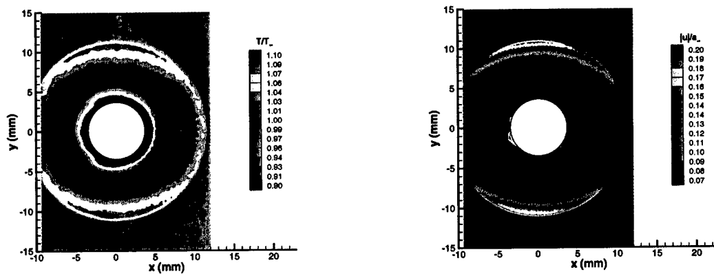
Figure 9: Temperature contours at t = 20\mu s for E = 145 mJ Figure 10: Velocity contours at t = 20\mu s for E = 145 mJ
