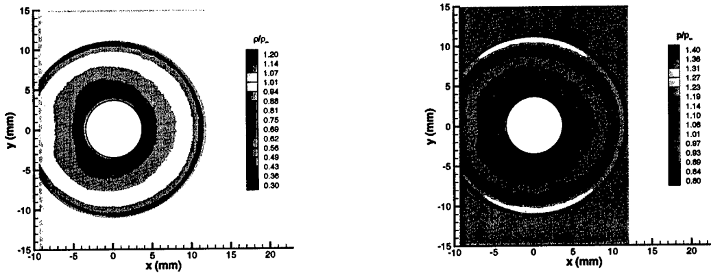
Figure 7: Density contours at t = 20\mu s for E = 145 mJ Figure 8: Pressure contours at t = 20\mu s for E = 145 mJ
