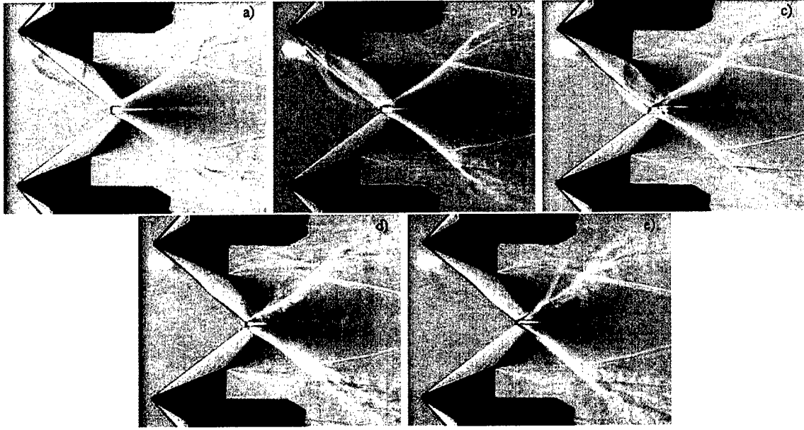
Figure 30: Experiment, a) t = 20 \mu s , b) t = 40 \mu s , c) t = 60 \mu s , d) t = 80 \mu s , e) t = 100 \mu s
