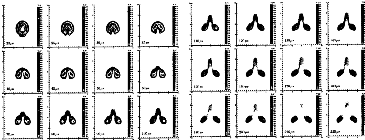
Figure 2: Time sequence of FRS temperature measurement ( E = 145 \text{ mJ} )
