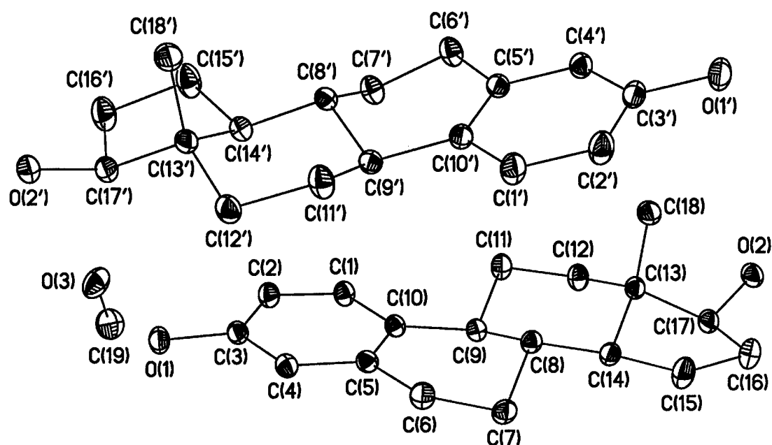
Figure 1. Thermal ellipsoid plot of 17 \beta -estradiol·½methanol where ellipsoids represent 50% probability electron density of the atom. Hydrogen atoms are omitted for clarity.
