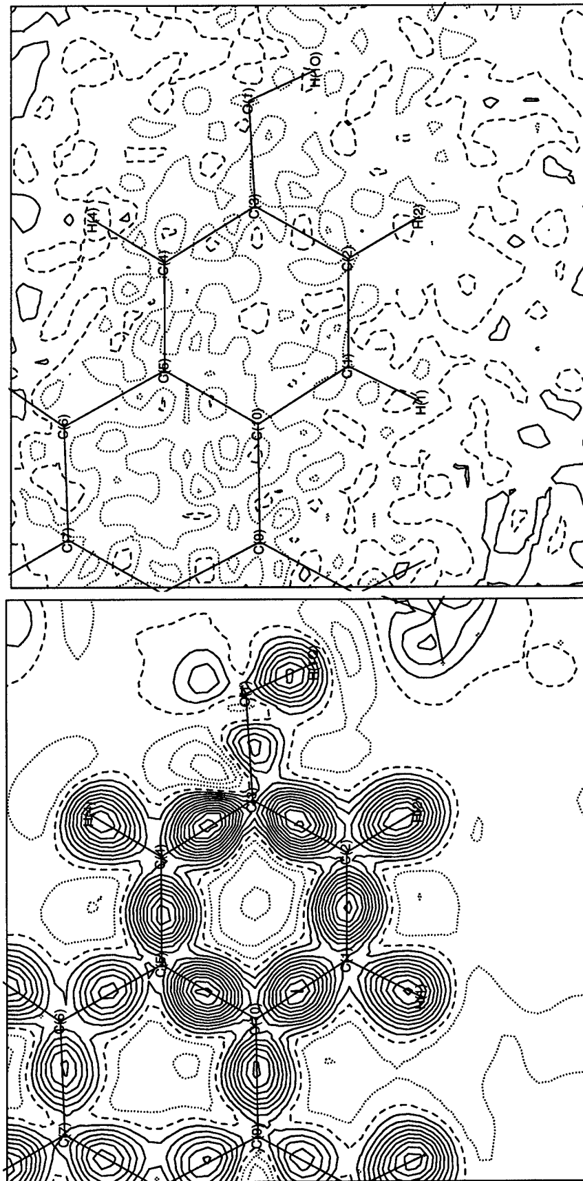
Figure 8. Dynamic model map and residual map in the plane of the aromatic ring of molecule 1 of 17\beta -estradiol• \frac{1}{2} methanol. Contour intervals are 0.05 \text{ e}\text{\AA}^{-3} with solid lines positive, dashed lines zero, and dotted lines negative.
