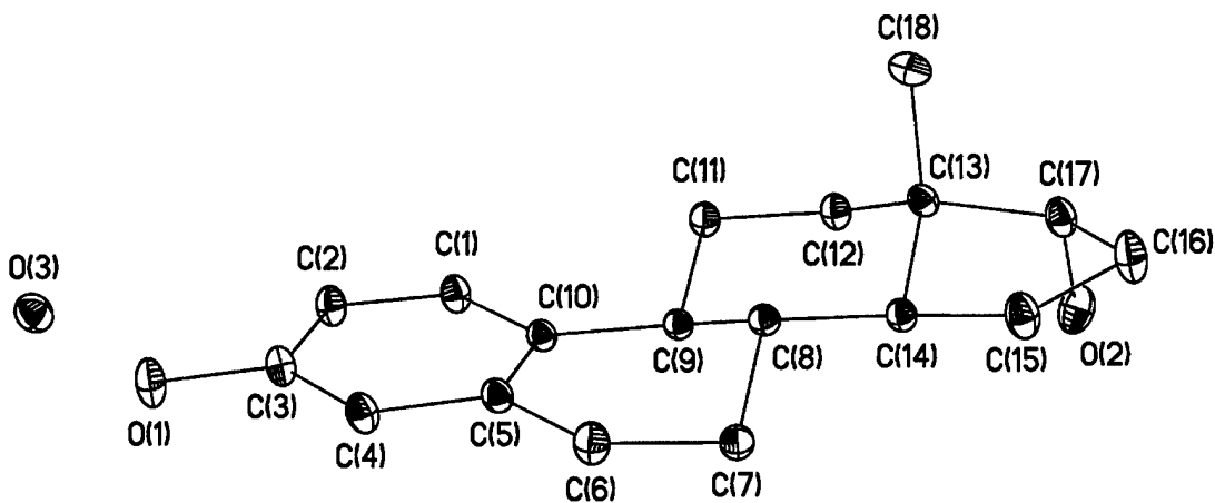
Figure 1. Thermal ellipsoid plot of 17α-estradiol·½H 2 O where ellipsoids represent 50% probability electron density of the atom. Hydrogen atoms are omitted for clarity.
