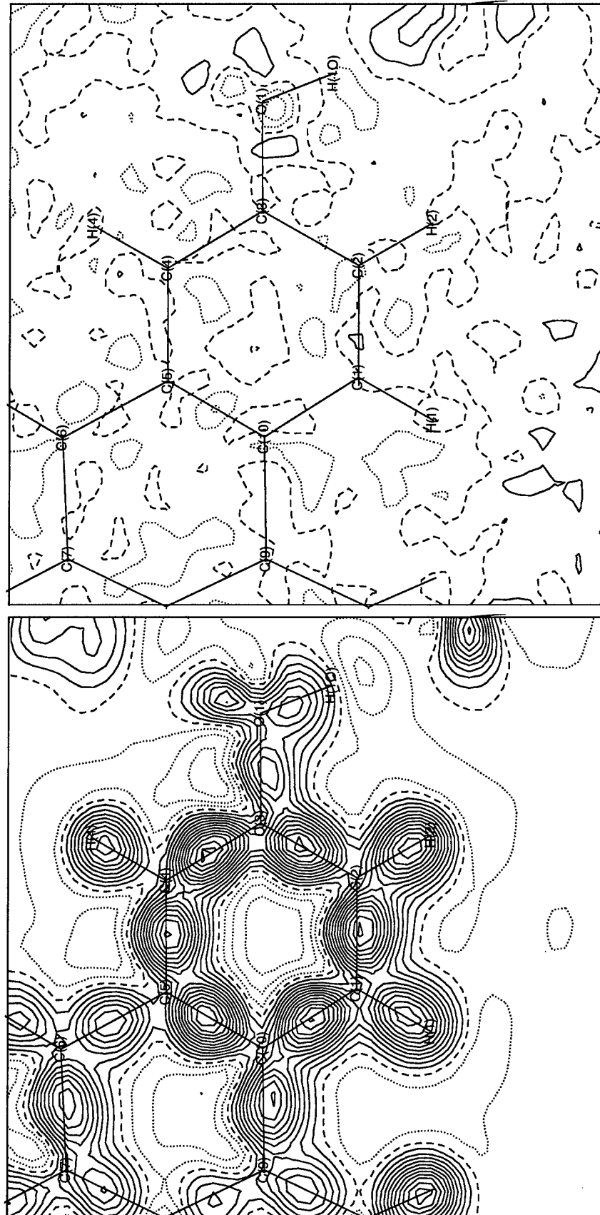
Figure 8. Dynamic model map and residual map in the plane of the aromatic ring of 17 \alpha -estradiol \cdot\frac{1}{2} H 2 O. Contour intervals are 0.05 eÅ -3 with solid lines positive, dashed lines zero, and dotted lines negative.
