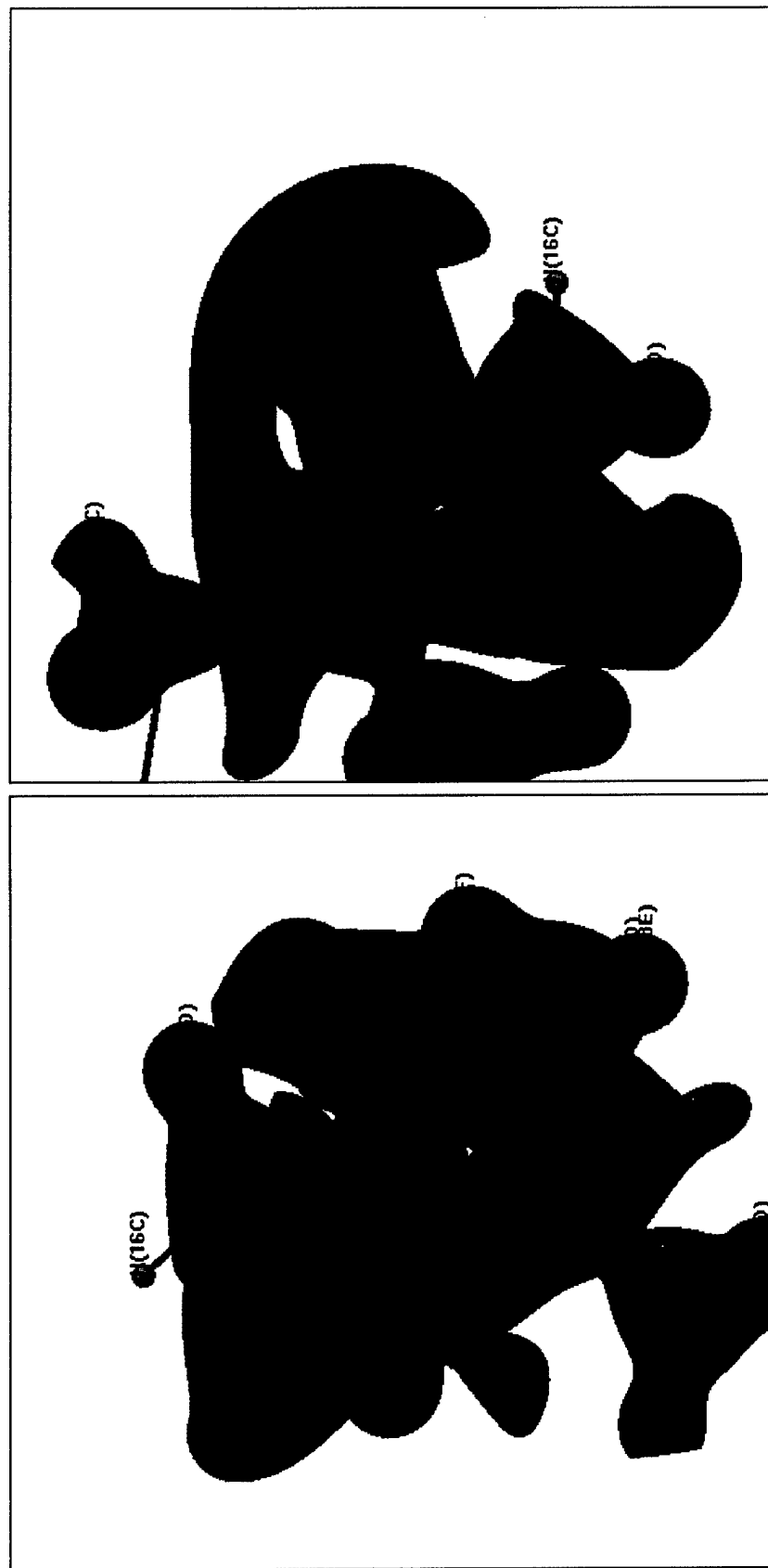
Figure 26. 17 \beta -estradiol 1:1 methanol, molecule 2 C17' hydroxy, red -0.15 eÅ -1 , blue 1.0 eÅ -1 .
