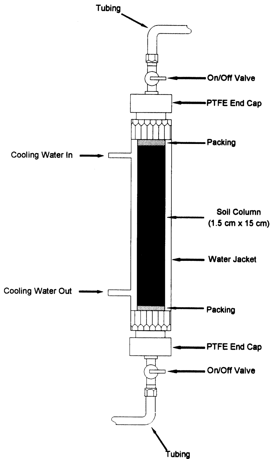
Figure 1. Design Schematic for the Column Reactors to be Used to Test Commercial Microbiological Amendments (drawing not to scale).
