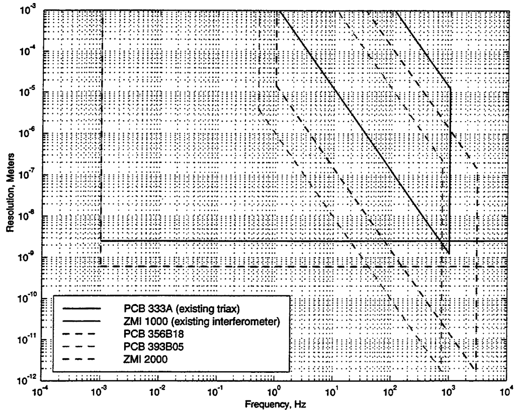
Figure 2-2 Resolution vs. frequency boundaries for the prior (solid) and acquired (dashed) instruments
