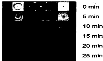
Figure 4: Time evolution of mixing in an electrohydrodynamically driven flow.
