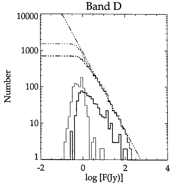
Figure 26: As for Figure 18, but for Band D.
