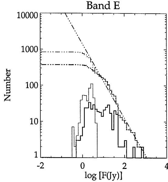
Figure 28: As for Figure 18, but for Band E.
