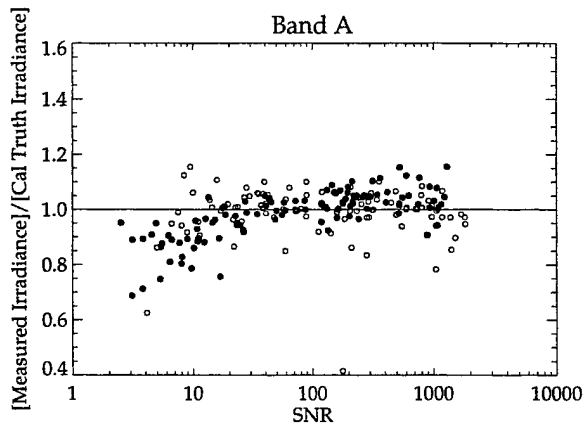
Figure 3: As for Figure 2, but for Bands A and C.
