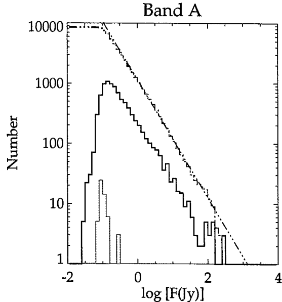
Figure 22: As for Figure 18, but for Band A.
