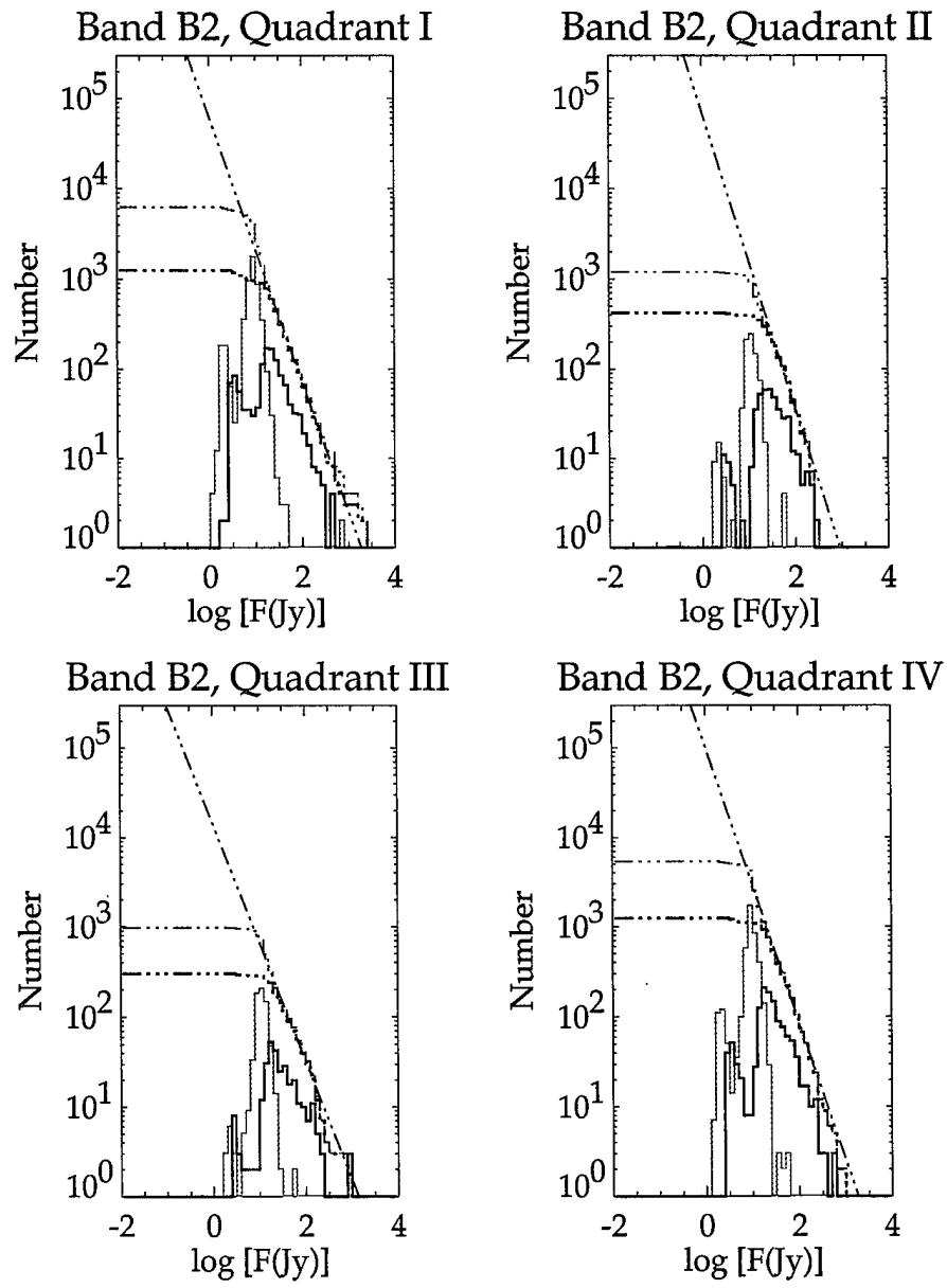
Figure 21: As for Figure 19, but for Band B 2 .
