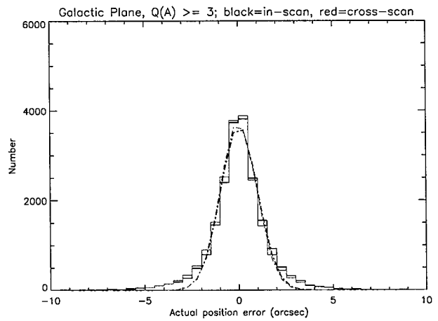
Figure 10: Position error (truth-measured) distribution of Galactic plane sources with (left) Q_A=2 and (right) Q_A \geq 3 .
