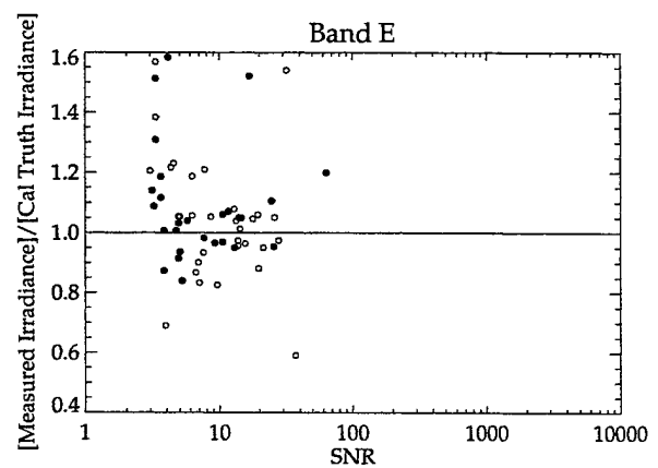
Figure 4: As for Figure 2, but for Bands D and E.
