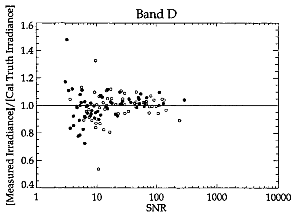
Figure 4: As for Figure 2, but for Bands D and E.
