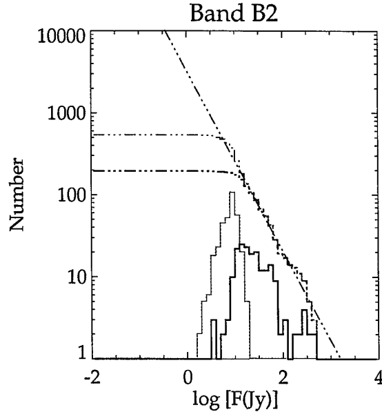
Figure 20: As for Figure 18, but for Band B 2
