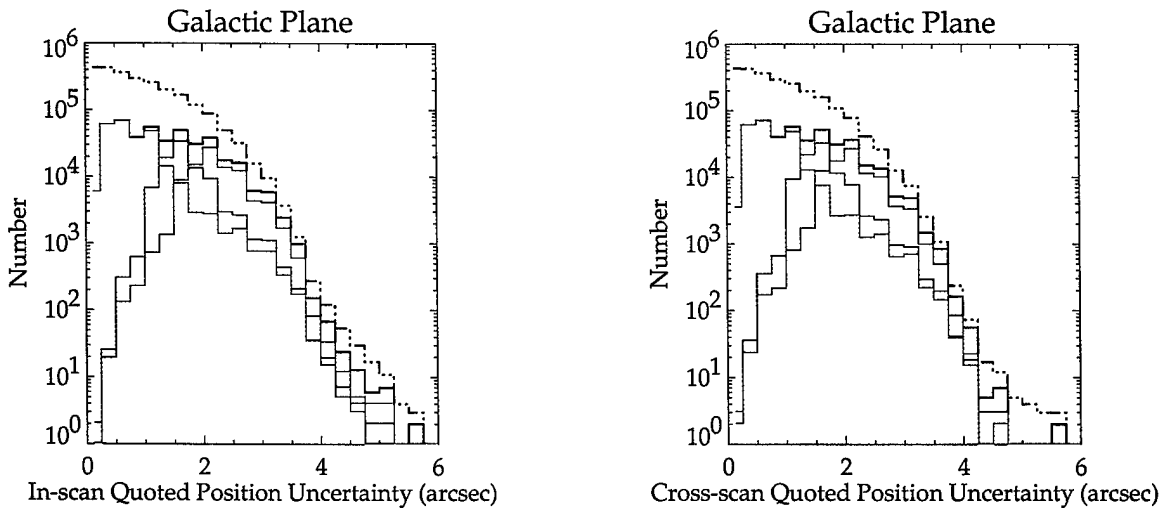
Figure 8: Quoted 1\sigma in-scan (left) and cross-scan (right) position uncertainties of the Galactic plane catalog sources.
