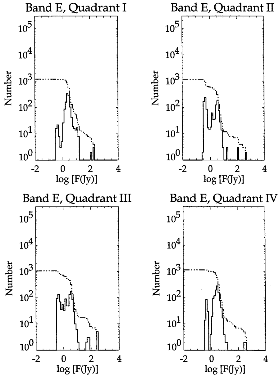
Figure 44: As for Figure 39, but for Band E.
