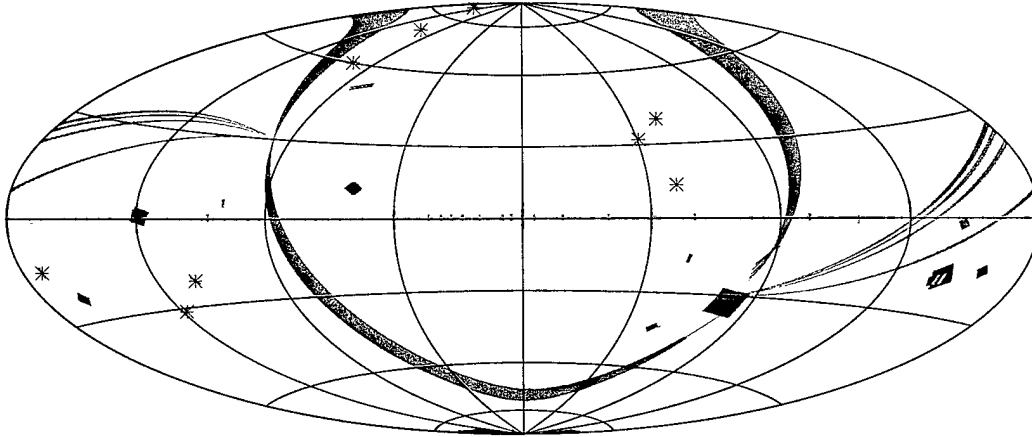
Figure 1: The areas surveyed by the MSX Celestial Background experiments. The map is an Aitoff equal-area projection in Galactic coordinates. The Galactic plane survey is shown in yellow, the Areas missed by IRAS in red, the five near Sun zodiacal scans in green, and the various raster scan observations of targeted areas in blue. Asterisks highlight those raster scans that did not cover a large enough area to show up on the plot.
