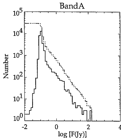
Figure 46: Band A source counts for PSC V1.2 with no counterpart in PSC V2.3.
