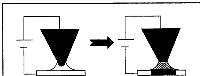
Figure 1. Schematic of the E-DPN modification of GaN nanowires. The AFM tip is first coated with KOH "ink" (blue) and engaged with the nanowire (yellow). During modification of the nanowire, KOH diffuses from the tip to the nanowire surface and electrochemically reacts with the nanowire to produce a gallium oxide heterostructure (green).
