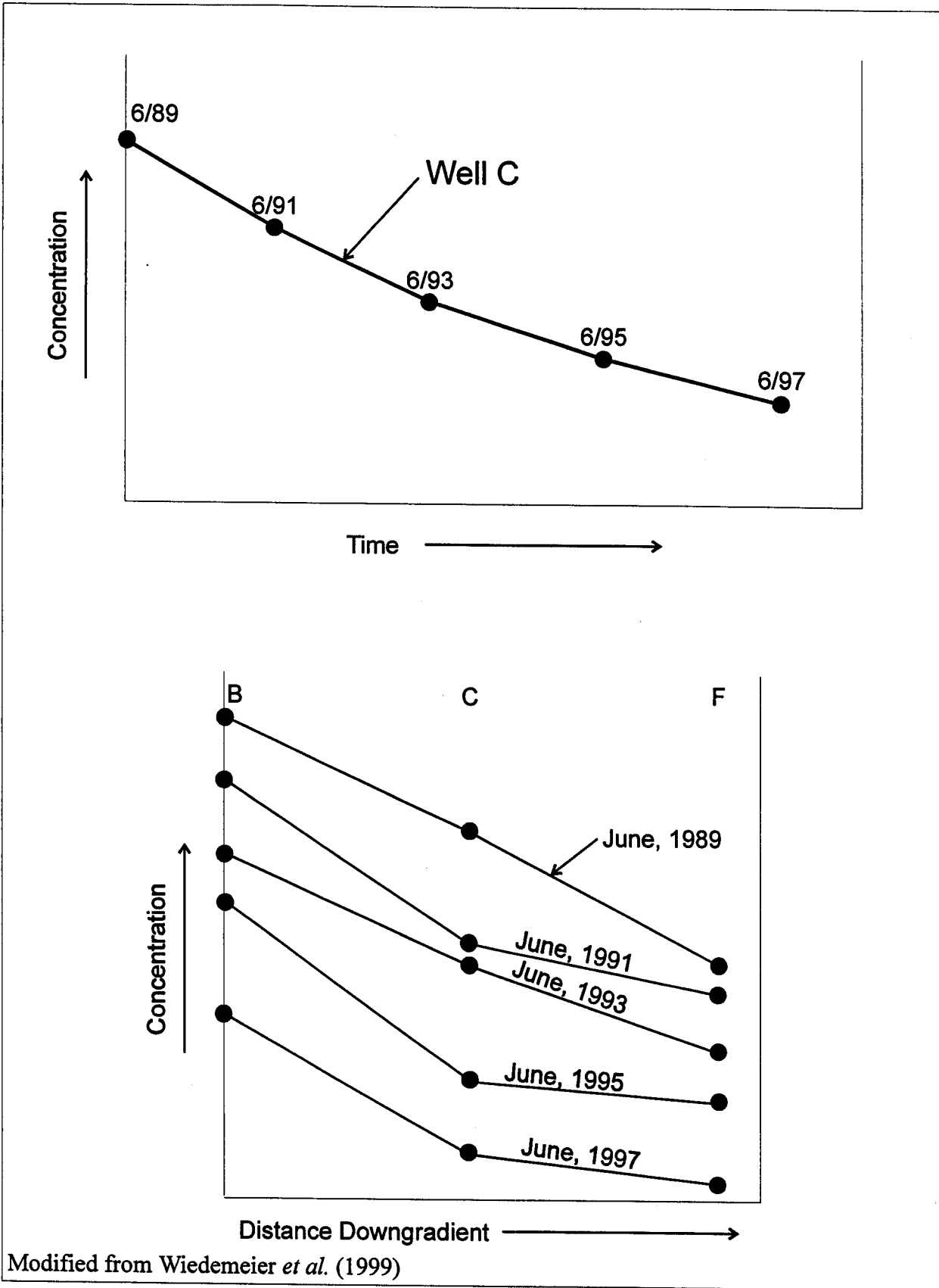
Figure 3.3b Plots of Contaminant Concentration Versus Time and Distance Downgradient
