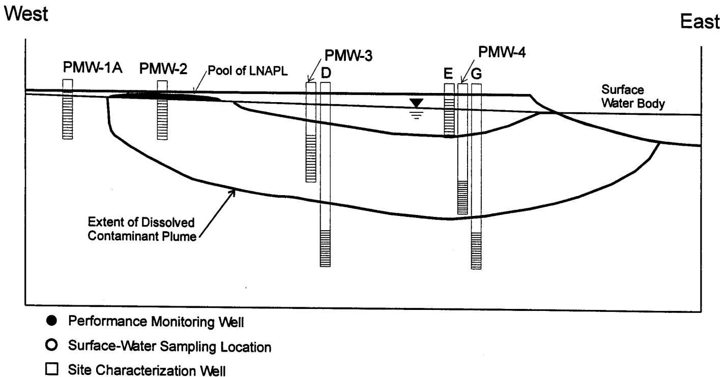
Figure 2.3 Locating Monitoring Wells and Surface Water Sampling Locations for a Discharging Plume (Modified from Wiedemeier et al. , 1999)
