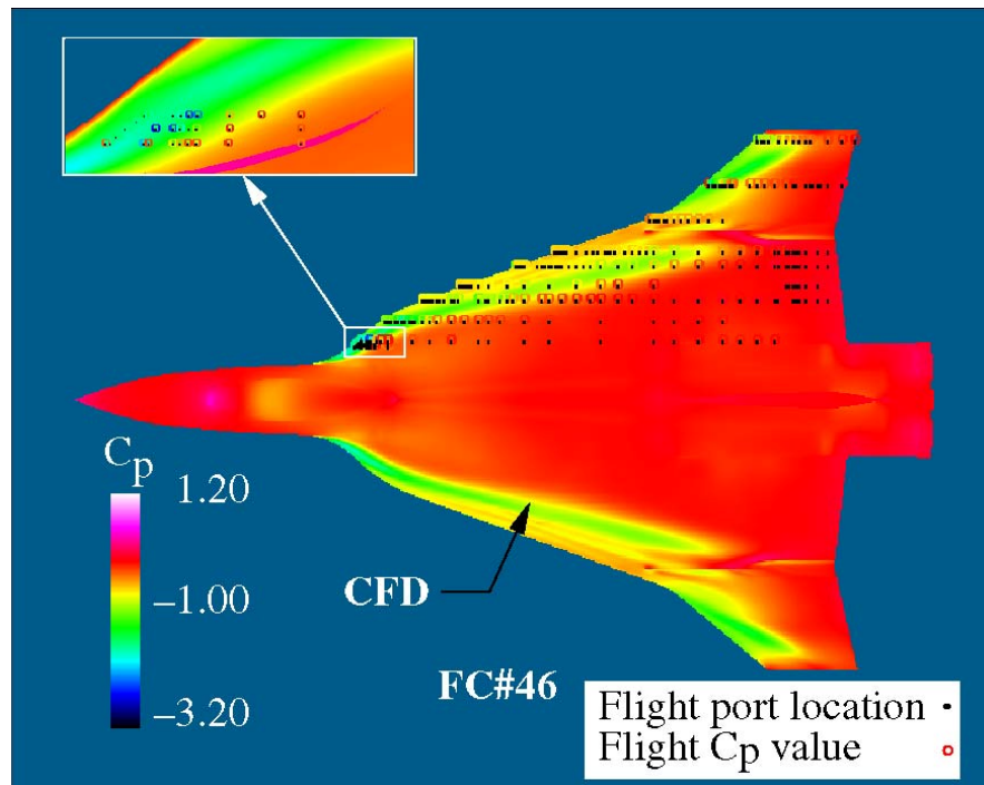
Figure 11. Predicted and measured flight C_{p,u} distribution of F-16XL-1 at FC#46 ( \alpha = 10.40^\circ ; M_\infty = 0.53 ; R_n = 46.90 \times 10^6 ).
