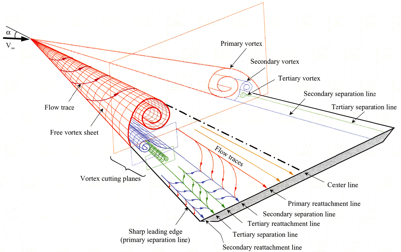
Figure 1. Anatomy of vortex flow on a delta wing at high angle of attack.
