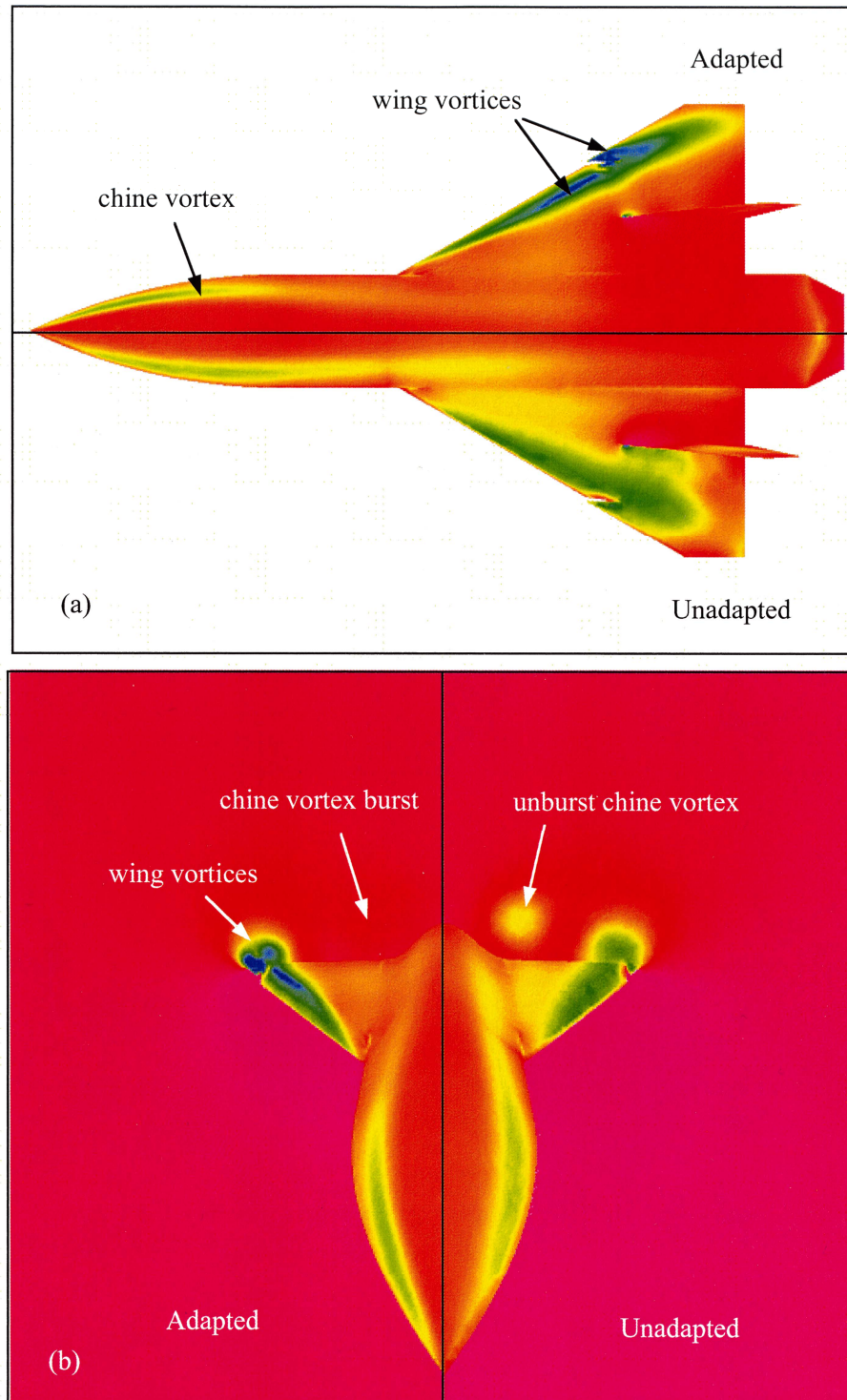
Figure 23. Initial and adapted static pressure distributions on the MTVI configuration: (a) surface and (b) surface/volume. M_\infty=0.4 , \alpha=20^\circ .
