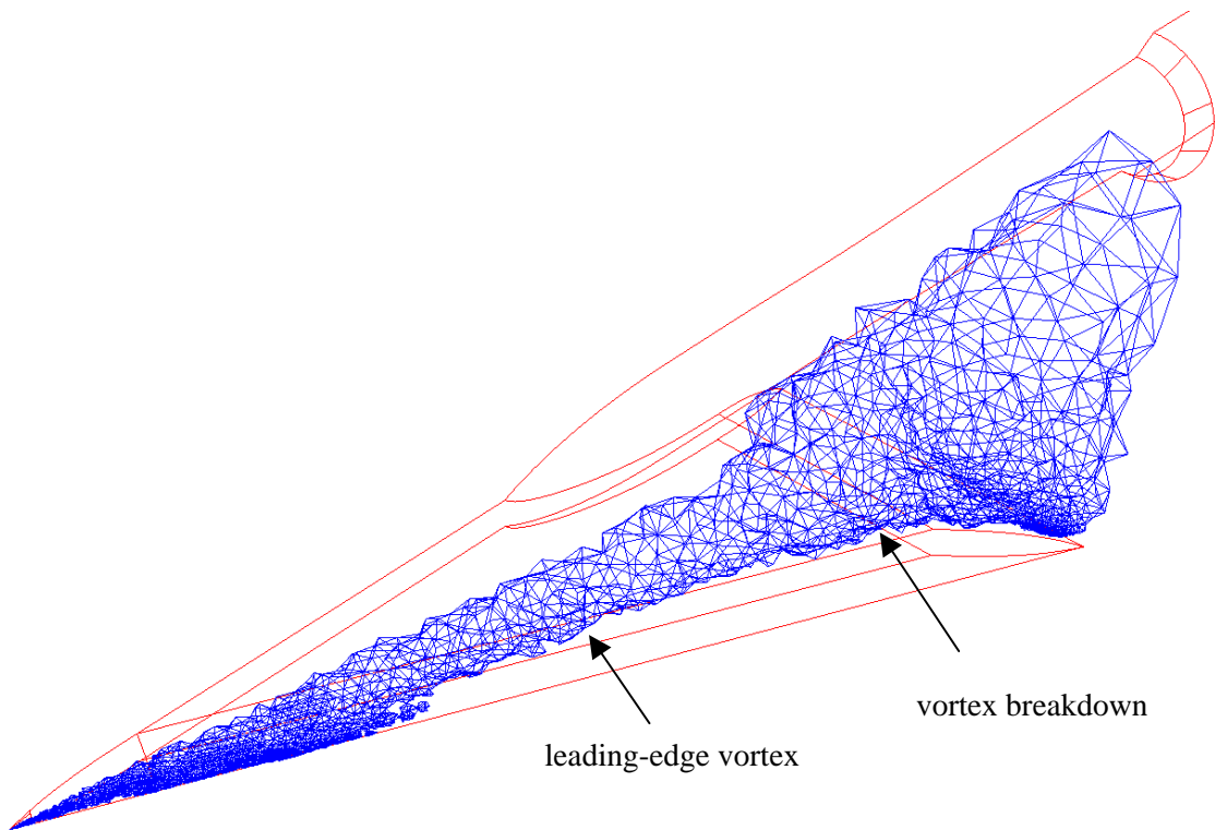
Figure 6. Adaptive grid refinement of high entropy region on initial grid for the sharp leading-edge Delta wing.
