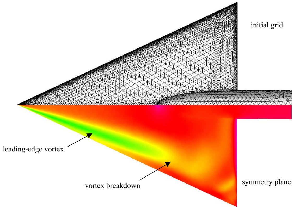
Figure 5. Initial (unadapted) grid (352,011 tetrahedral cells) and Euler inviscid flow solution on the sharp leading-edge Delta wing. M_\infty=0.4 , \alpha=20^\circ .
