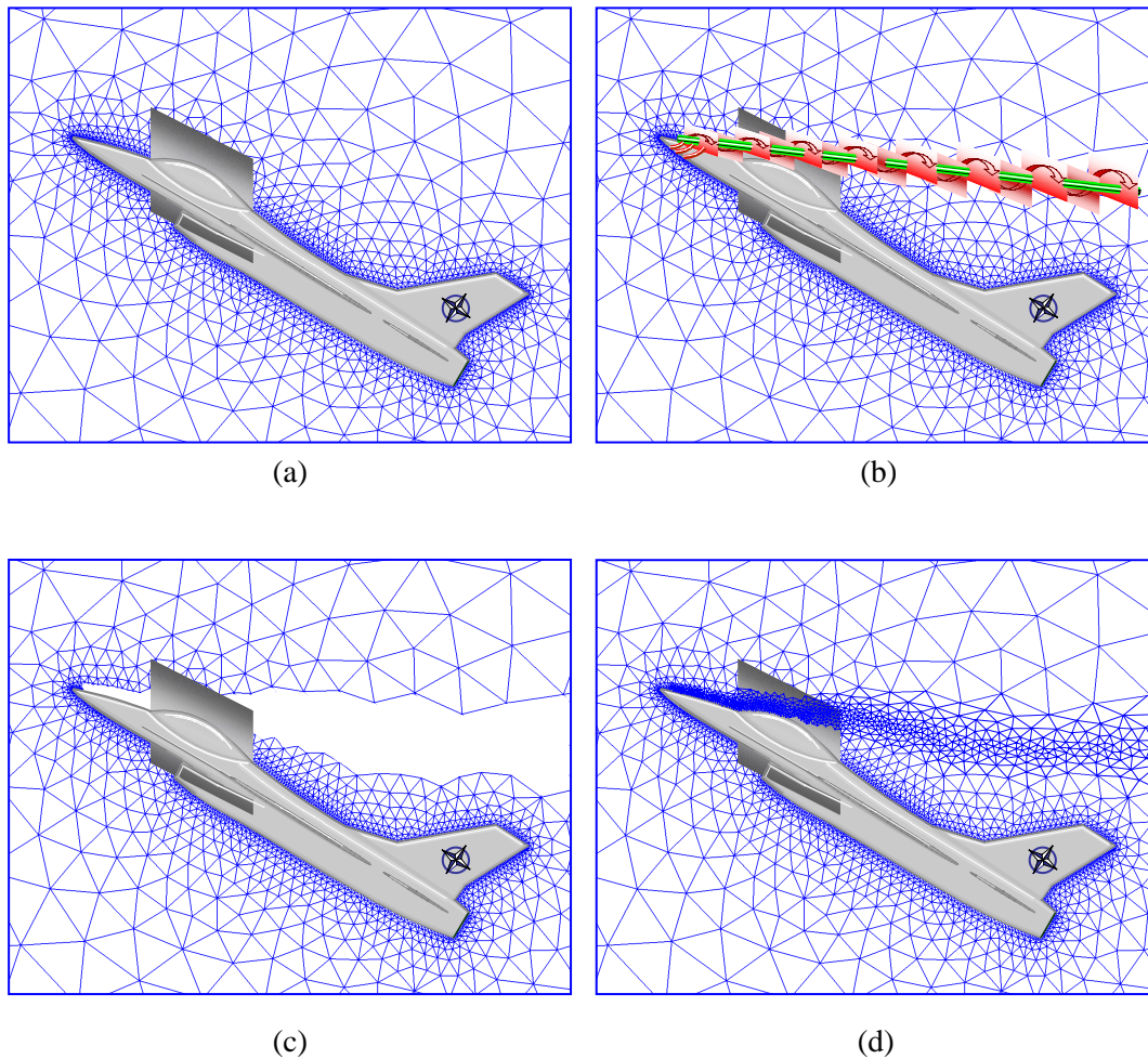
Figure 2. Demonstration of adaptive refinement steps by local remeshing for a vortical flow example: (a) initial grid, (b) flow solution indicating a forebody vortex, (c) removal of affected cells, and (d) locally refined grid.
