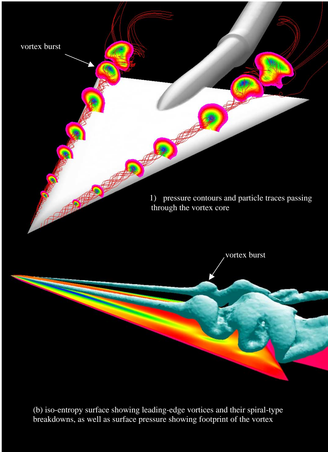
Figure 9. Adapted Euler inviscid flow solution on the sharp leading-edge Delta wing. M_\infty=0.4 , \alpha=20^\circ .
