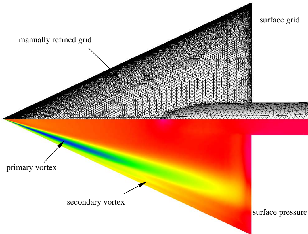
Figure 10. Unadapted refined grid (2,720,797 cells) and Navier-Stokes flow solution on the sharp leading-edge Delta wing. M_\infty=0.4 , \alpha=20^\circ , Re_{MAC}=6.0 \times 10^6 .
