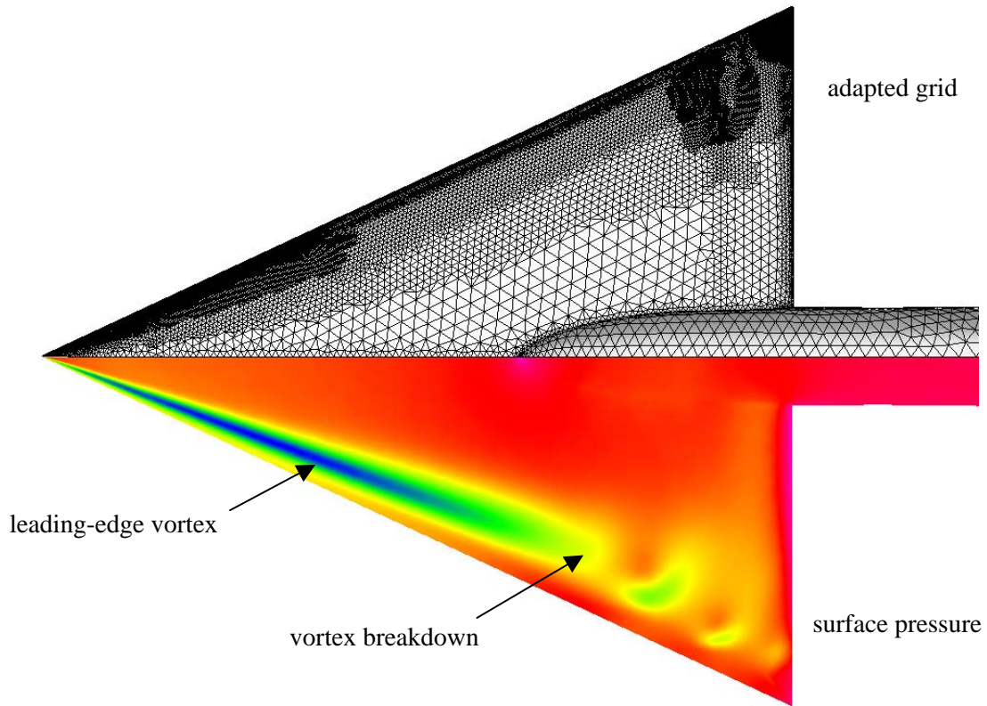
Figure 7. Final adapted grid (1,612,307 cells) and Euler inviscid flow solution on the sharp leading-edge Delta wing. M_\infty=0.4 , \alpha=20^\circ .
