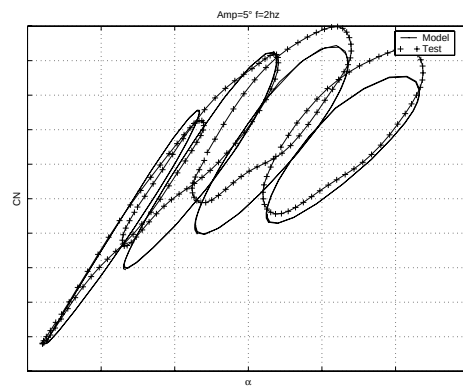
figure 7 : Comparison between test and model (simplified « knowledge model »)
