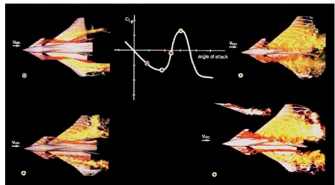
Fig 13 Lateral instability due to asymmetric vortex bursting
