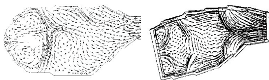
(a) vaporiser type (b) airspray type Fig 9 Combustion chamber internal flows
