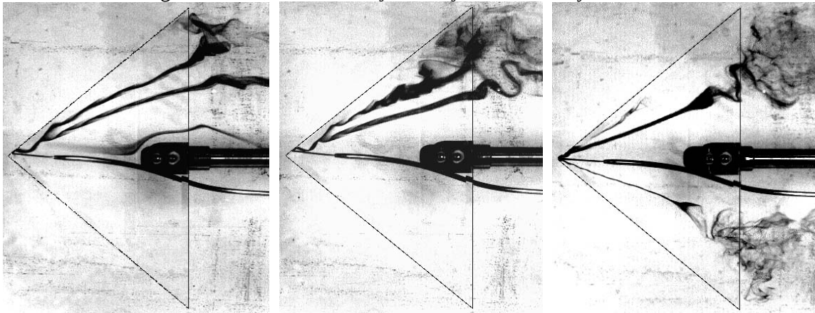
Figure 6. Evolution of secondary LEV: \alpha = 5^\circ, 7.5^\circ , and 10^\circ , 50° wing
