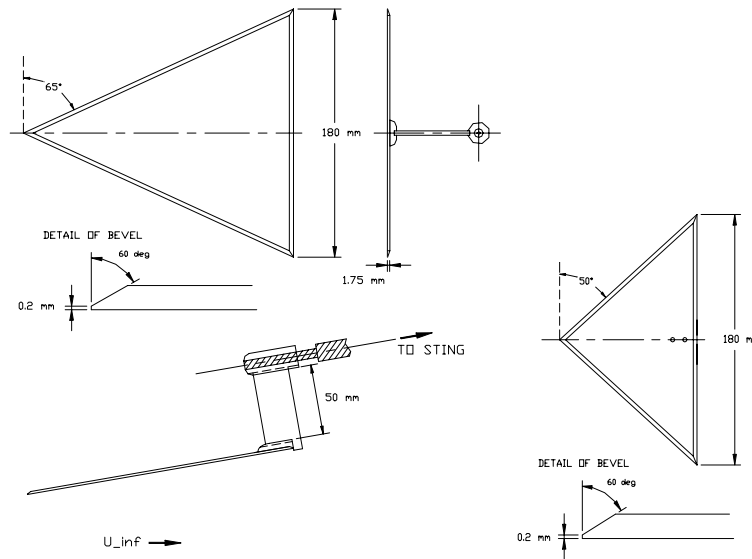
Figure 1. 65° and 50° wing models, with mounting arrangement
