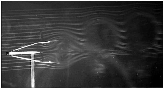
Fig. 10: Centerline wake topology at k=1.5 .
