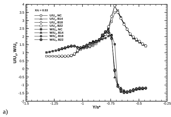
Fig. 4: U/U_\infty and W/U_\infty profiles at Q_m = 0, 1.4\text{g/s}, 1.8\text{g/s} and 2.2\text{g/s} (NC, B14, B18 and B22). Profile locations of (a) X/c=0.53 (b) X/c = 0.63 .
