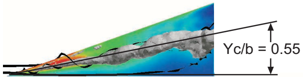
Fig. 22: Instantaneous contours of surface pressure and an iso-surface of entropy in the vortex core at maximum suction, Y_c/b=0.55 . ( \alpha=35^\circ , Re=200,000 )
