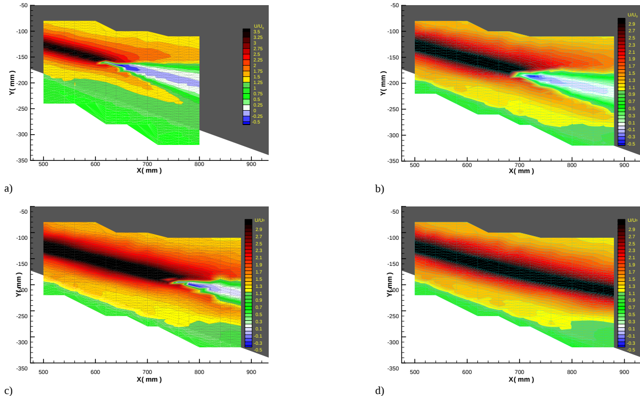
Fig. 3: LDV results of U/U_\infty in the longitudinal plane at \alpha = 27^\circ and U_\infty = 24 m/s. Portside along-the-core blowing with Q_m = (a) 0 (b) 1.4 g/s. (c) 1.8 g/s (d) 2.2 g/s.
