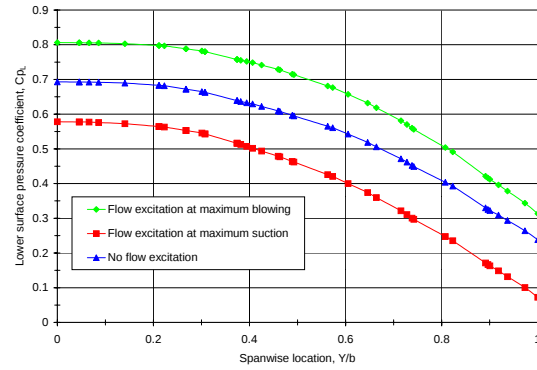
Fig. 12: Pressure distribution on the lower surface of the wing. Sample results at X/C=0.3 .
