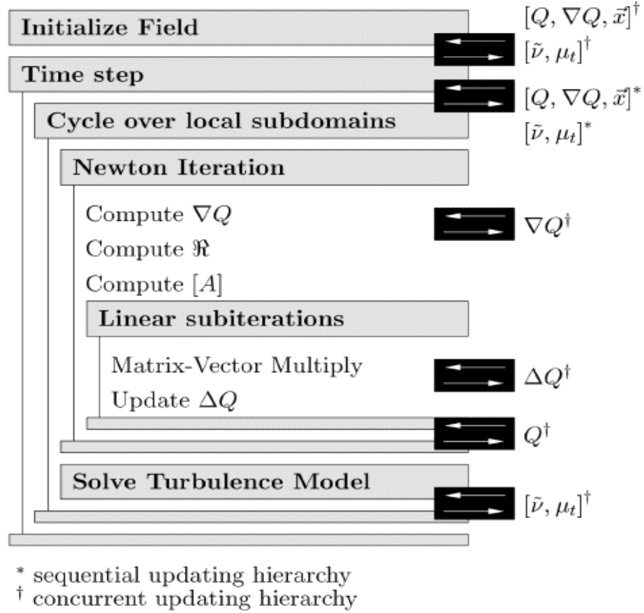
Figure 2: Iteration Hierarchy
