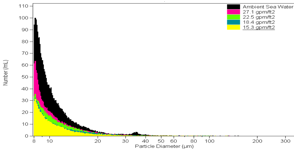
Figure 27. Particle size distributions in seawater passed through Anthracite (0.95 to 1.05 mm) at various loading rates.
