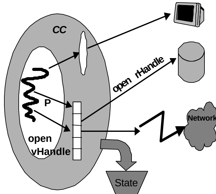
Figure 4: Handle virtualization
