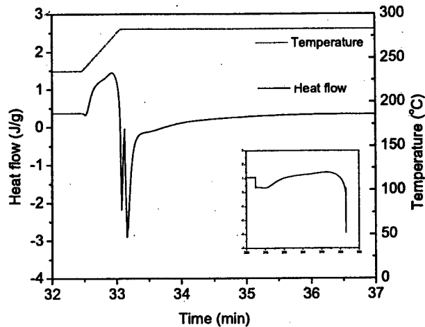
Figure 9 DSC curve showing the first peak reaction at a high heating rate of 80^{\circ}\text{C}/\text{min}
