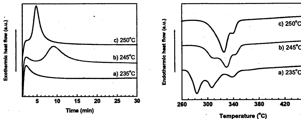
Figure 5 Isothermal annealing of gas atomized Al_{85}Ni_{10}La_5 powders.
