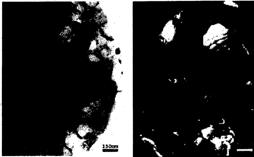
Figure 12 Powder particles ( <25\ \mu\text{m} ) that heat-treated for 250^\circ\text{C} for 6 hrs and followed by a holding at 268^\circ\text{C} for 6 hrs: (a) Bright field (Left); and (b) Dark field (Right).
