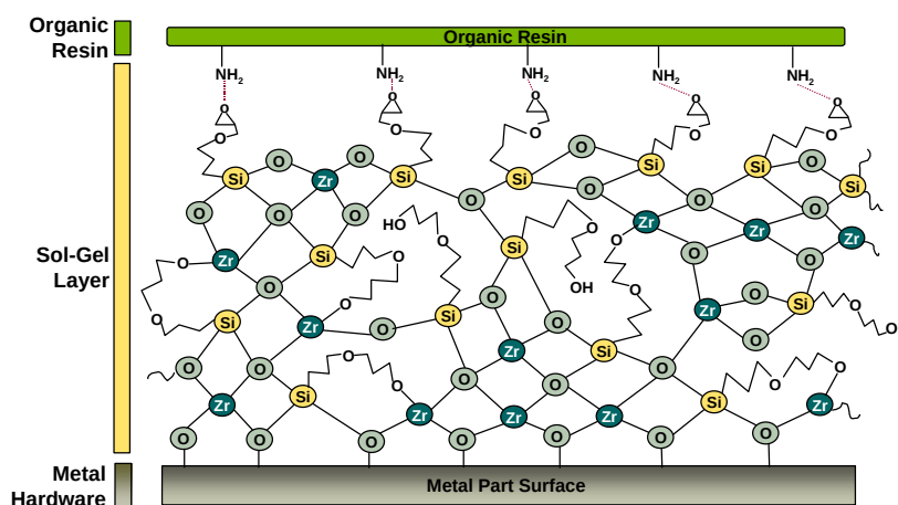
Figure 2.1-1 Notional Schematic of Sol-Gel Adhesion-Promoting Coating on a Metal Part
