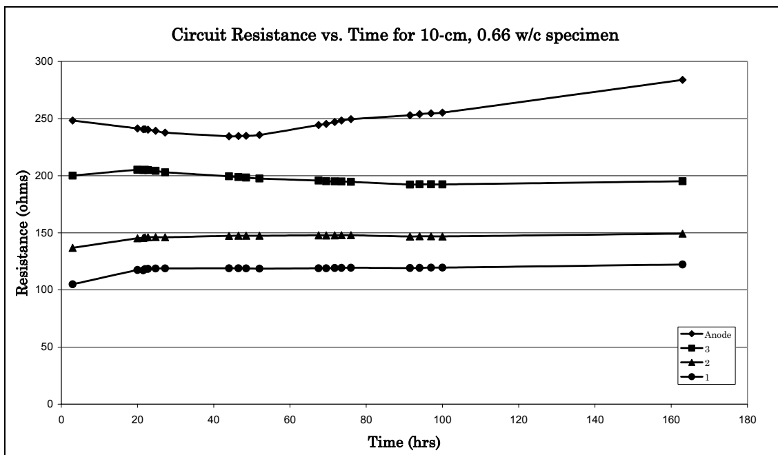
Figure 22. Resistance vs. time (0.66 w/c).
