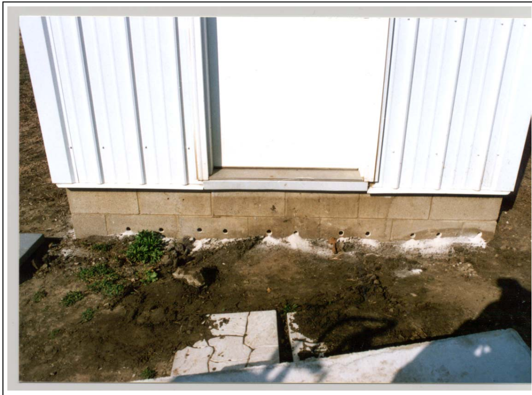
Figure 52. East wall of block basement with above-grade holes drilled to fill wall with grout.
