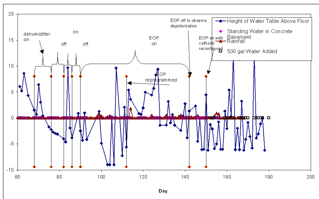
Figure 45. Water table and standing water in concrete basement.
