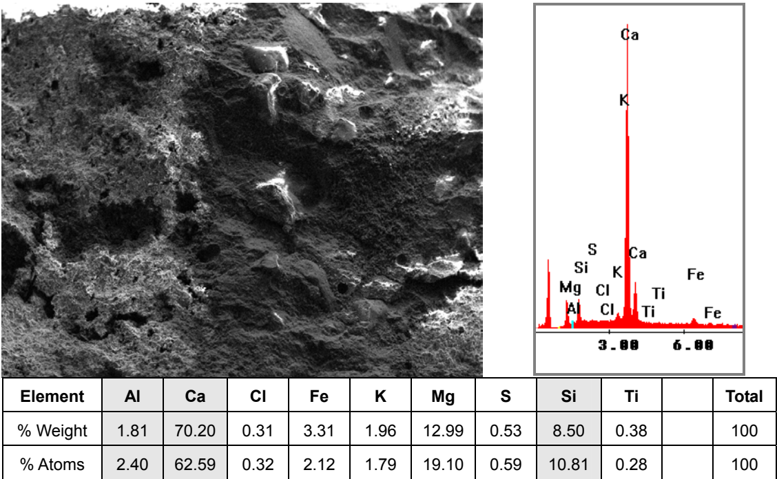
Figure 31. SEM analysis of 0.63 w/c specimen before electro-osmosis experiment. (Row values may not total 100 due to rounding.)
