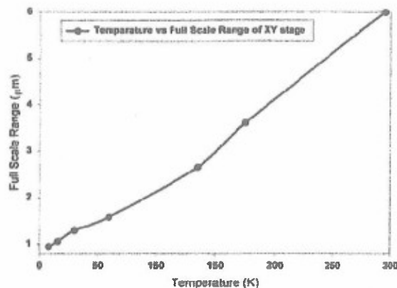
Figure 39. Calibration of the scanning stage for the Low
