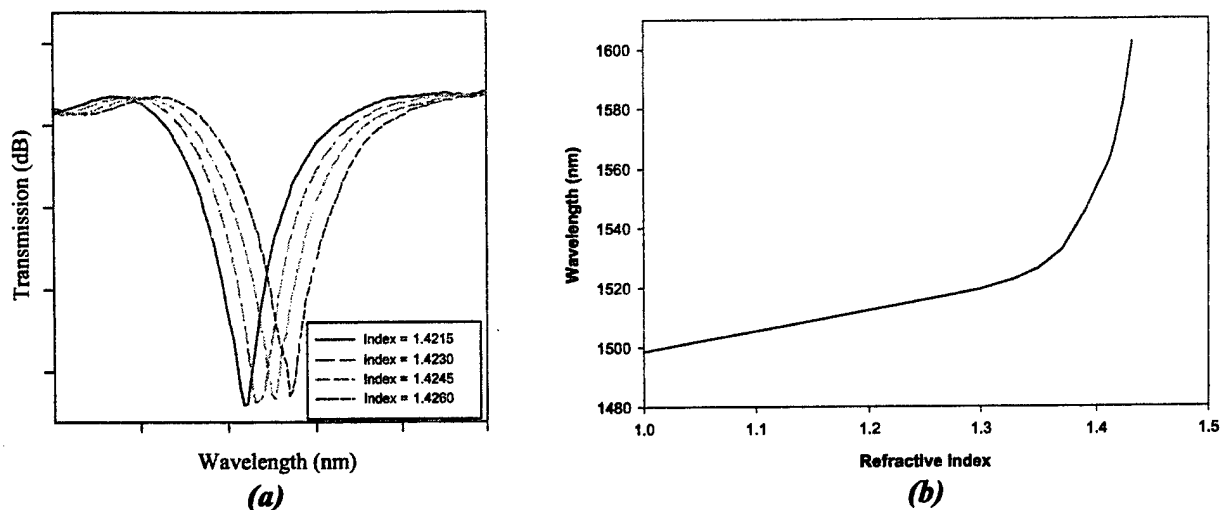
Figure 5 a) Typical LPG transmission spectrums for different refractive index solutions. b) LPG response to refractive index change is asymptotic. Maximum refractive index resolution is seen in the higher (>1.35) refractive index range.
