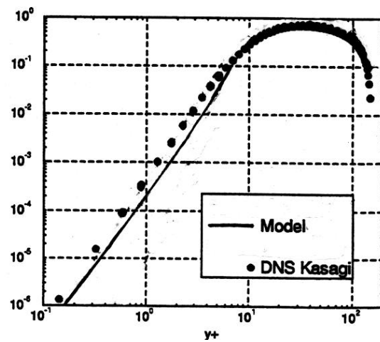
Fig.4 : Dimensionless turbulent heat flux -v\theta^+
