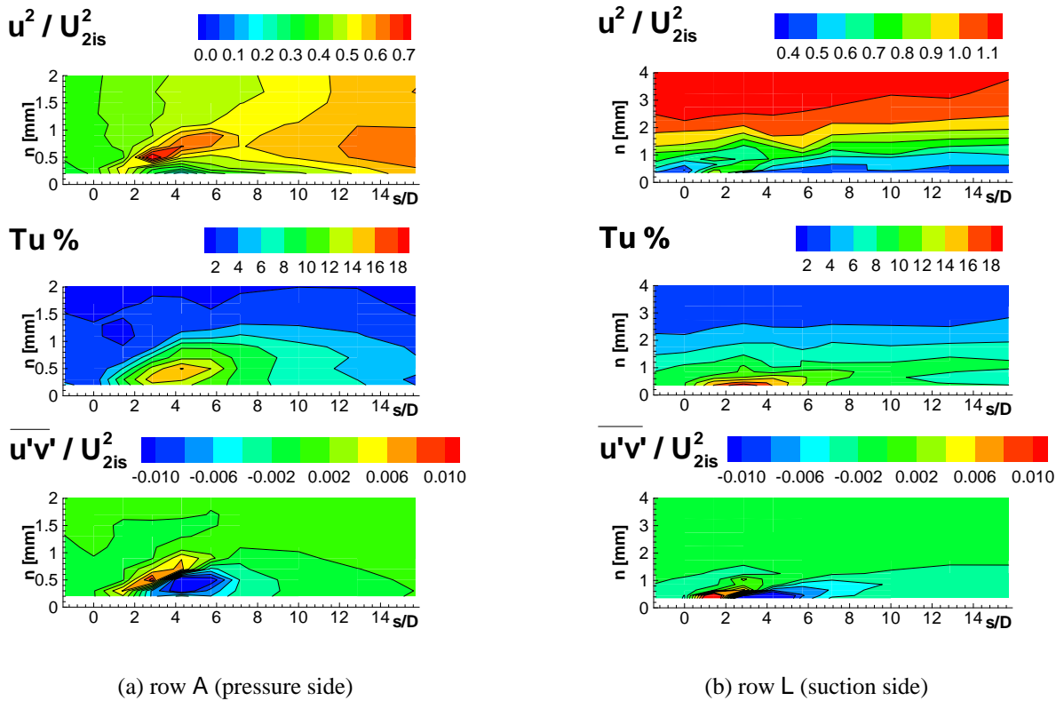
Figure 12: Hole centerline flow characteristics in the s, n plane.
