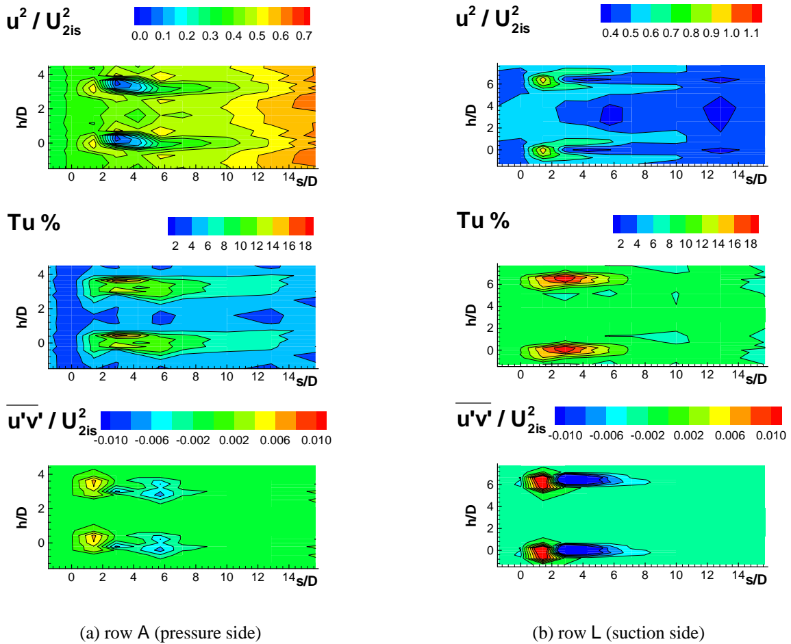
Figure 11: Flow characteristics in the s, h plane closest to the wall.
