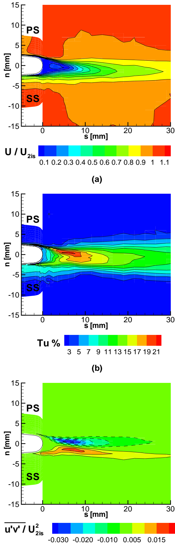
Figure 5: The near wake flow field
