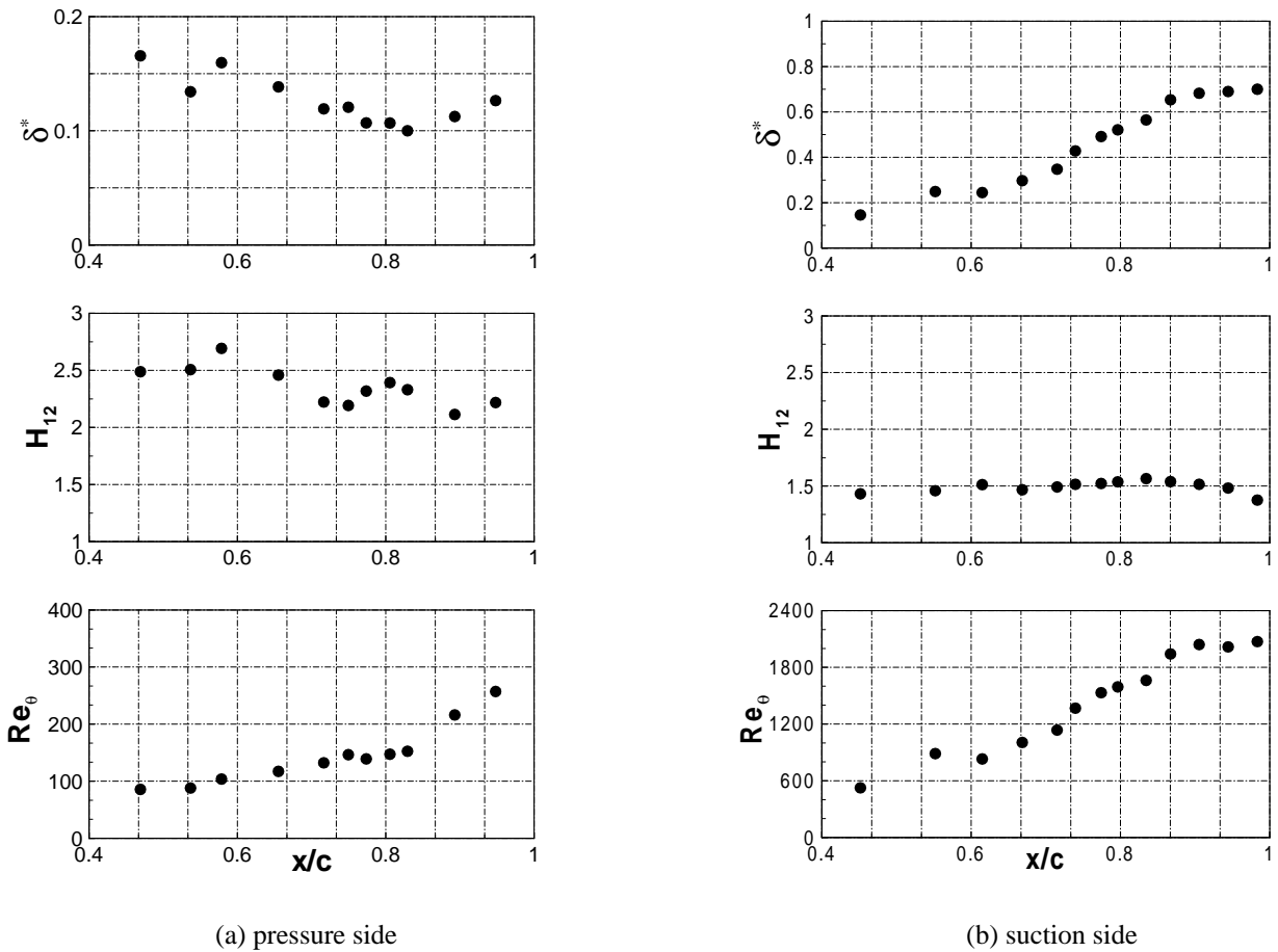
Figure 7: Integral parameters.
