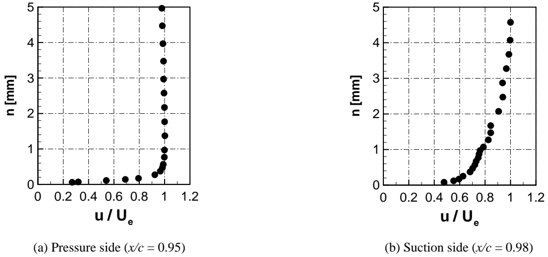
Figure 6: Boundary layer profiles close to the trailing edge.
