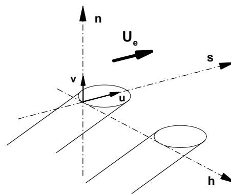
Figure 2: Hole coordinate system.
