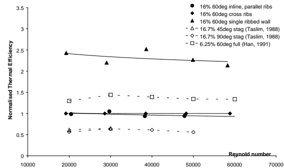
Figure 16 Comparison of the normalized thermal efficiency of the ribbed wall between different configurations
