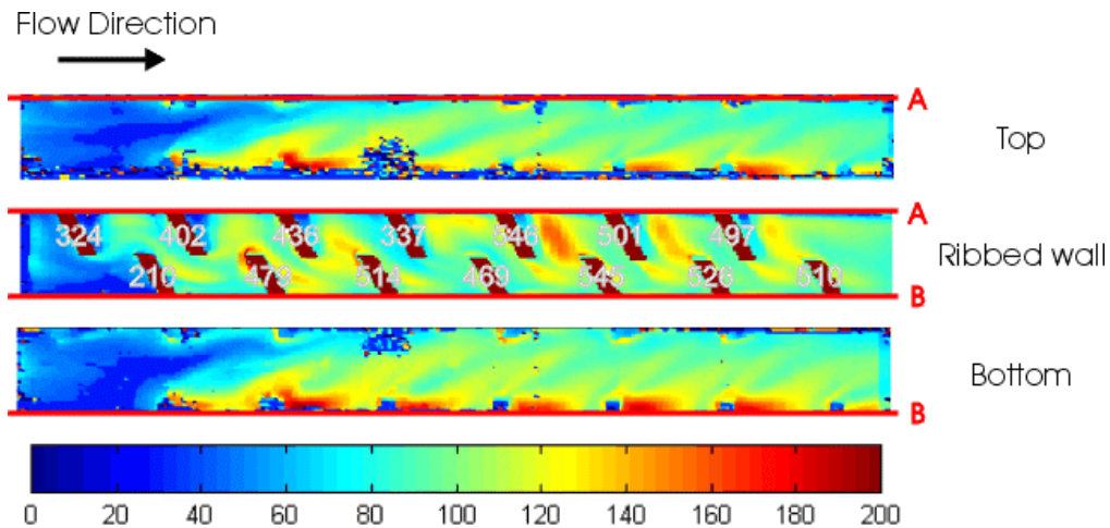
Figure 8 Htc distribution for configuration B at Re 50,000
