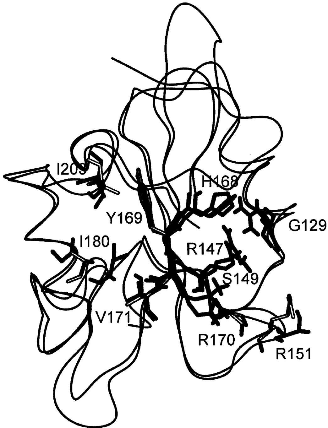
Figure 5: The superposition of the phosphopeptide binding site of the CHK-SH2 domain (red, PDB id#:1JWO) and v-Src SH2 domain (blue, PDB id#:1BKL). Residues involved in binding pTyr ( G^{129} , R^{147} , H^{168} , R^{170} ) are indicated in red for CHK and in blue for the corresponding residues of Src. Residues comprising the hydrophobic site that interact with residues comprising the C-terminal to pTyr region of the phosphopeptide are indicated in pink (CHK) and in green (Src). The nonconserved R^{151} of CHK is indicated in pink.
