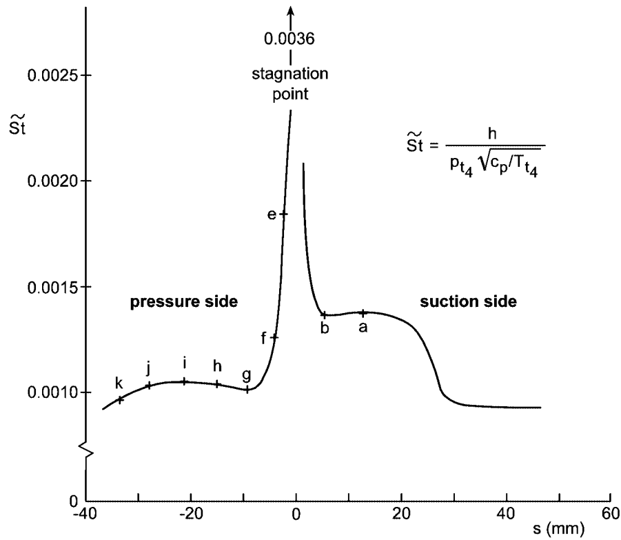
Fig. 9 Stanton number distribution on rotor blade at engine design point
