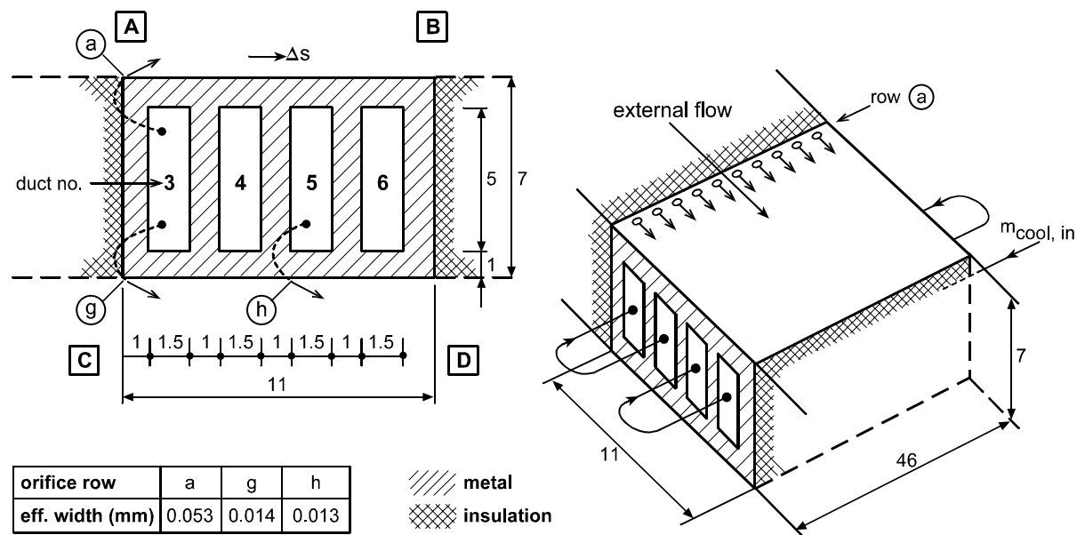
Fig. 10 Configuration to demonstrate coupled heat transfer analysis
