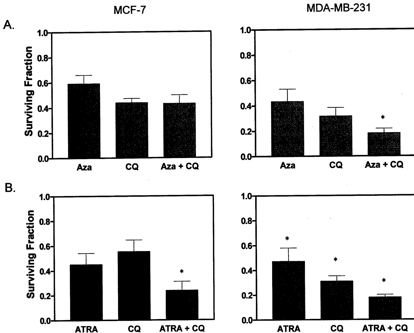
Figure 3A,B: Effect of Chloroquine antimalarial \pm 5-Aza-dC or ATRA on tumor clonogenic survival. 6 \times 10^3 MCF-7 or MDA-MB-231 cells pretreated with CQ ( 33 \mu\text{M} ), 5-Aza-dC ( 1 \mu\text{M} ), or ATRA ( 1 \mu\text{M} ) were plated in 5ml of 10% FBS DMEM in 60mm dish plates. MCF-7 and MDA-MB-231 cells were then subjected to a 7 or 5 day (undisturbed) incubation period, respectively. To visualize colonies, dishes were stained with 3 ml of 0.5% crystal violet, 5% formalin, 50% ethanol, 0.85% NaCl for 3 minutes, then rinsed with tap water. Colonies were scored using a Nikon Eclipse TS100 microscope at 20X magnification with \geq 20 MCF-7 cells and \geq 50 MDA-MB-231 cells = 1 colony. Data represents n=3 (duplicates per each individual experiment) \pm SEM (* p < 0.001 ).
