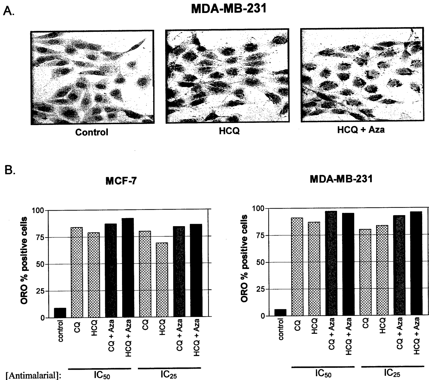
Figure 4A,B: Oil-Red-O (ORO) Histochemistry: Effect of Chloroquine or Hydroxychloroquine antimalarials ± 5-Aza-dC on cellular differentiation. A.) HCQ (IC 25 ) ± 10μM 5-Aza-dC B.) CQ or HCQ (IC 50 and IC 25 ) ± 10μM 5-Aza-dC. MCF-7 and MDA-MB-231 cells were plated on 5x5 mm 2 95% ethanol-washed glass coverslips in 35 mm 2 dishes at 2x10 5 and 1x10 5 cells per dish, respectively. 48 hours after drug treatment, the ORO assay was performed and lipid droplet accumulation in the cytoplasm was visualized by light microscopy. At least 300 cells were counted visually. Data represents 1 experiment.
