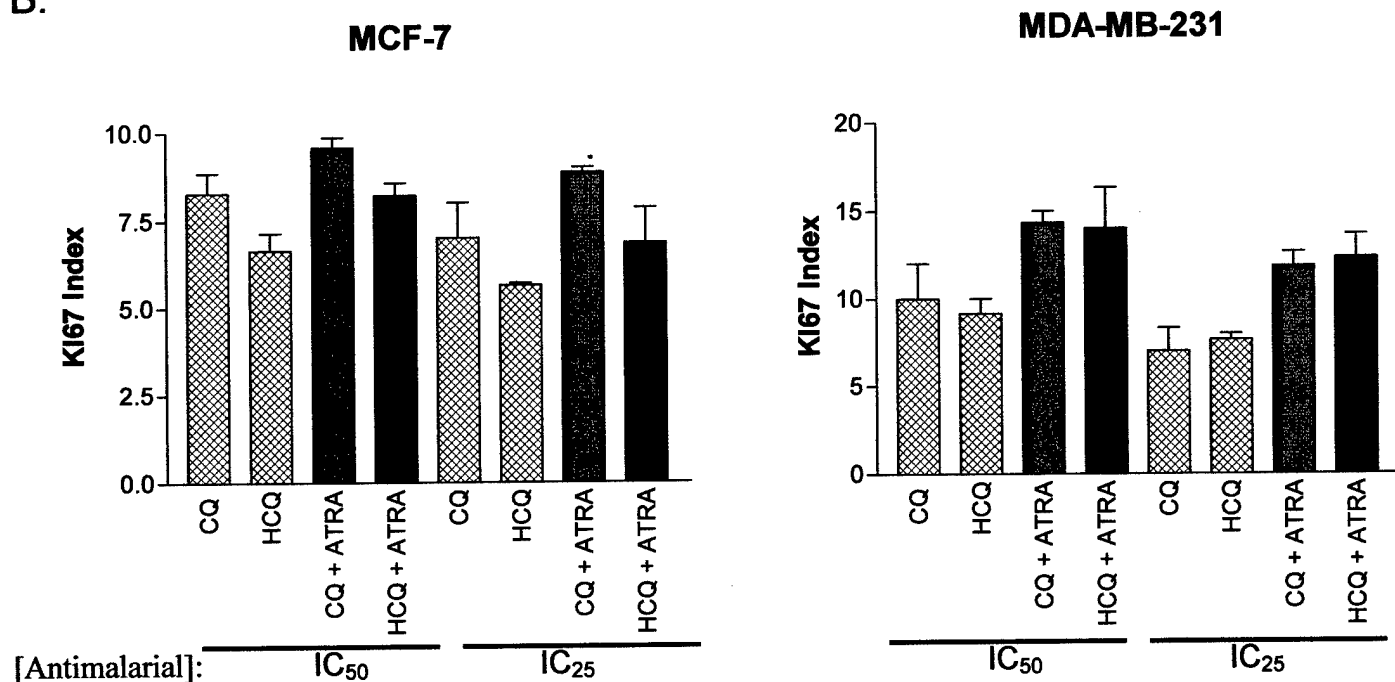
Figure 6A,B: KI67 Histochemistry: Effect of Chloroquine or Hydroxychloroquine antimalarials ± 5-Aza-dC or ATRA on cellular differentiation. A.) CQ or HCQ (IC 50 and IC 25 ) ± 10 \mu M 5-Aza-dC; n=1 B.) CQ or HCQ (IC 50 and IC 25 ) ± 10 \mu M ATRA; n=2 (+/- SEM). MCF-7 and MDA-MB-231 cells were plated on 5x5 mm 2 95% ethanol-washed glass coverslips in 35 mm 2 dishes at 2x10 5 and 1x10 5 cells per dish, respectively. 48 hours after drug treatment, KI67 immunohistochemistry was performed. KI67 negative percentage of the cell population was determined by visual counting. At least 500 cells were counted. (KI67 Index=%KI67 negative drug treated/ %KI67 negative control).
