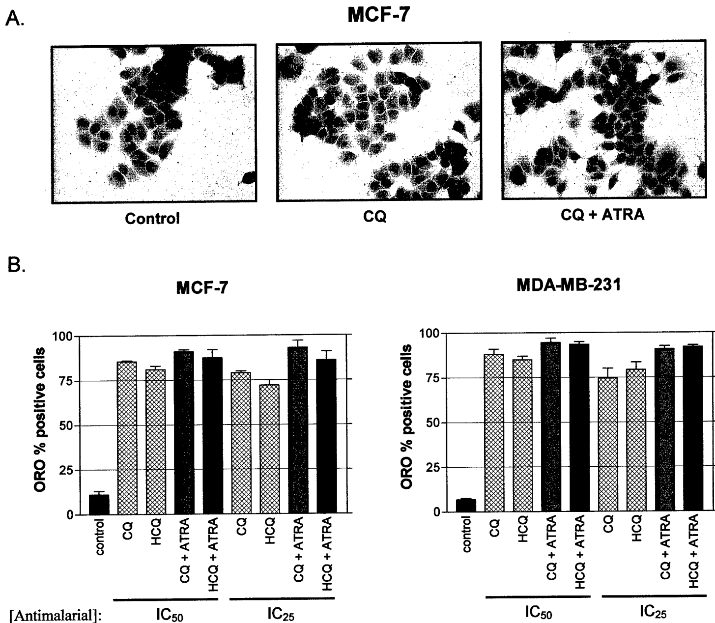
Figure 5A,B: Oil-Red-O (ORO) Histochemistry: Effect of Chloroquine or Hydroxychloroquine antimalarials ± ATRA on cellular differentiation. A.) CQ (IC 25 ) ± 10µM ATRA B.) CQ or HCQ (IC 50 and IC 25 ) ± 10µM ATRA. MCF-7 and MDA-MB-231 cells were plated on 5x5 mm 2 95% ethanol-washed glass coverslips in 35 mm 2 dishes at 2x10 5 and 1x10 5 cells per dish, respectively. 48 hours after drug treatment, the ORO assay was performed and lipid droplet accumulation in the cytoplasm was visualized by light microscopy. At least 300 cells were counted visually. Data represents the mean of 2 independent experiments (+/- SEM).
