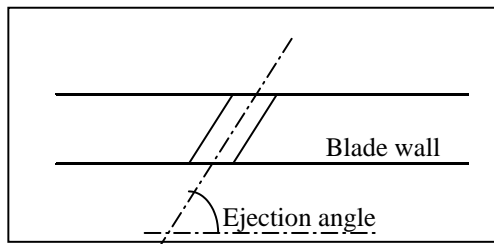
Figure n°5 : Film cooling geometry
