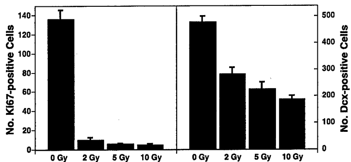
Fig. 8: Numbers of proliferating cells (left) and immature neurons (right) in the dentate SGZ are significantly decreased 48 hr after irradiation. Each bar represents an average of 4 mice; error bars are SEM.
