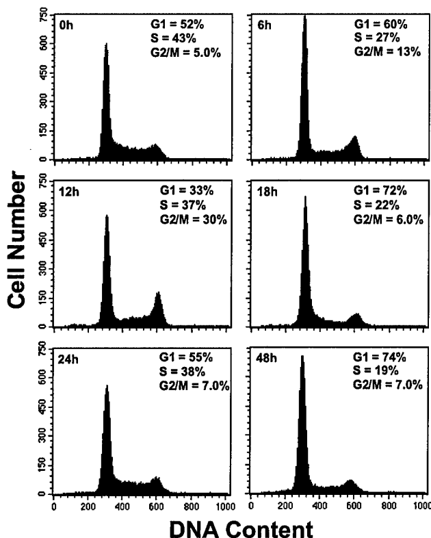
Fig. 1: Activation of cell cycle checkpoints after x-irradiation. Histograms illustrate functional G2/M and G1/S checkpoints as evidenced by the pronounced buildup of cells in the G2/M (12 hr) and G1 (18 h) cell cycle compartments, respectively
