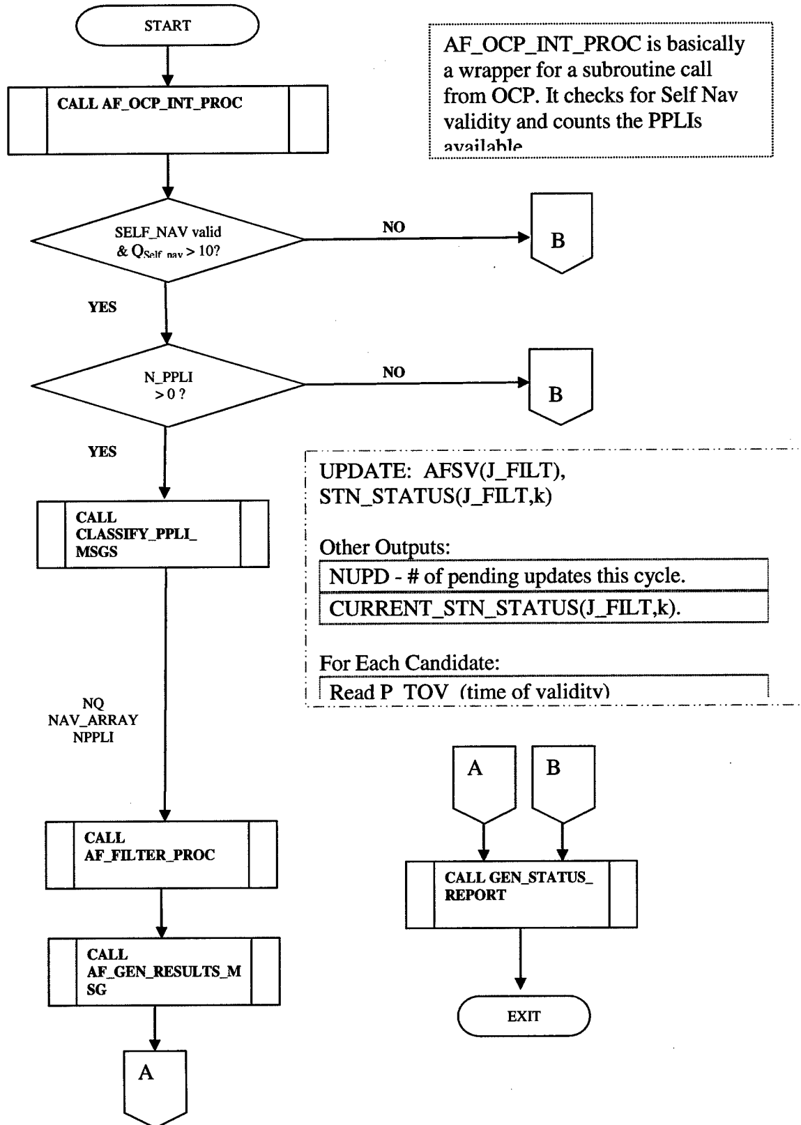
Figure 89 AF_EXEC_CTRL PROCESSING: LEVEL 2 Flowchart
