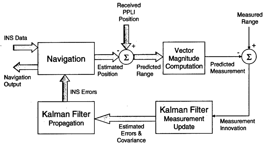
Hybrid Navigation Diagram
