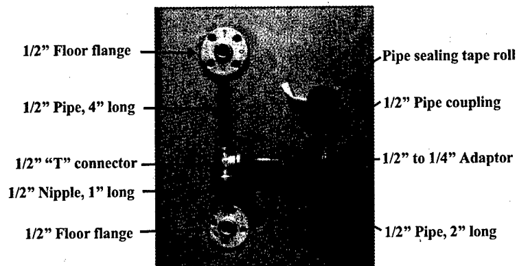
Air pipe unit parts
