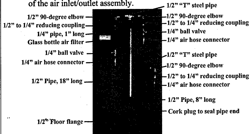
Air inlet/outlet assembly parts
