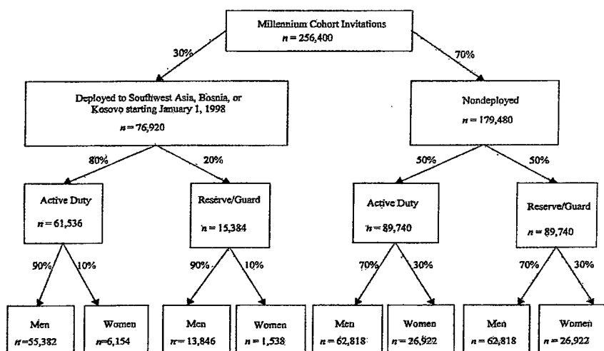
Figure 1: Sampling Strategy.
