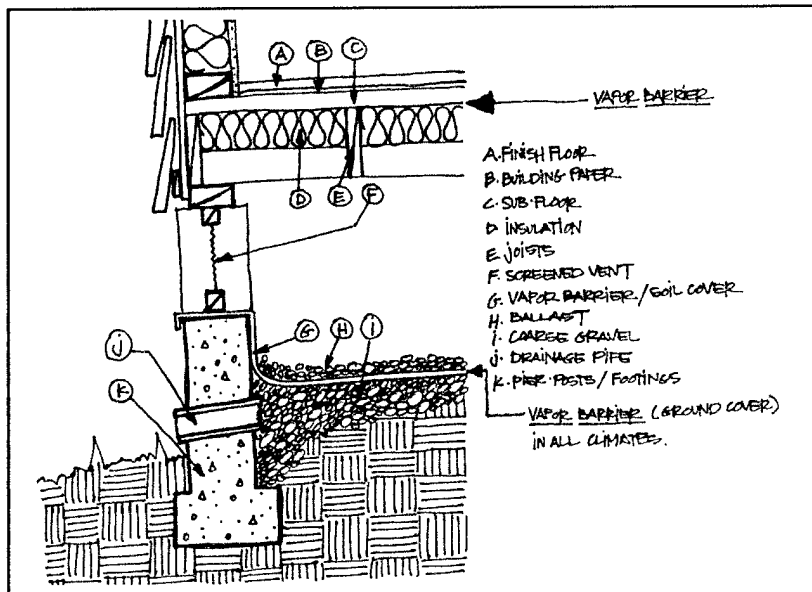
Figure 2, Adapted standard crawl-space detail from FPL (1949) and Ramsey and Sleeper (1992).
