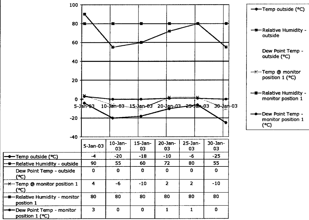
Figure 3.6, Spruce Siding, with vapor barrier, in Minneapolis, in January with air conditioning. Outside temperature, relative humidity – outside, Dew Point data at monitor position 1, and relative humidity – monitor position 1 obtained from WUFI (2003). Dew Point data obtained from Stein B. and Reynolds, J. (1992).
