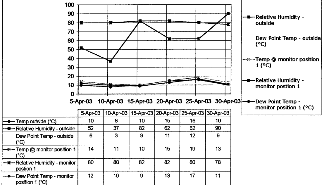
Figure 3.3, Spruce Siding, without vapor barrier, in Roanoke, in April with air conditioning. Outside temperature, relative humidity – outside, Temperature at monitor position 1, and relative humidity – monitor position 1 obtained from WUFI (2003). Dew Point data obtained from Stein B. and Reynolds, J. (1992).
