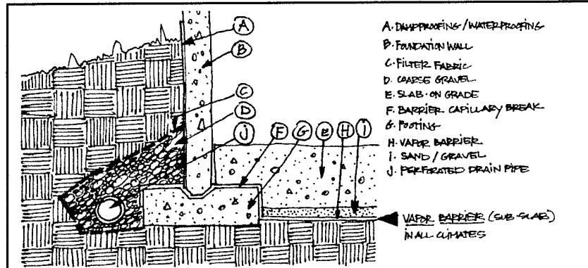
Figure 1, Adapted standard slab-on-grade and basement detail from Ramsey and Sleeper (1992).
