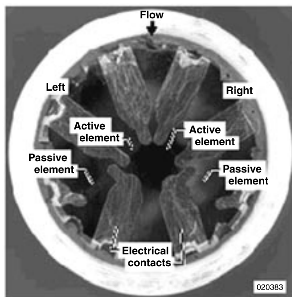
(b) High temperature dual hot-film sensor [62].
