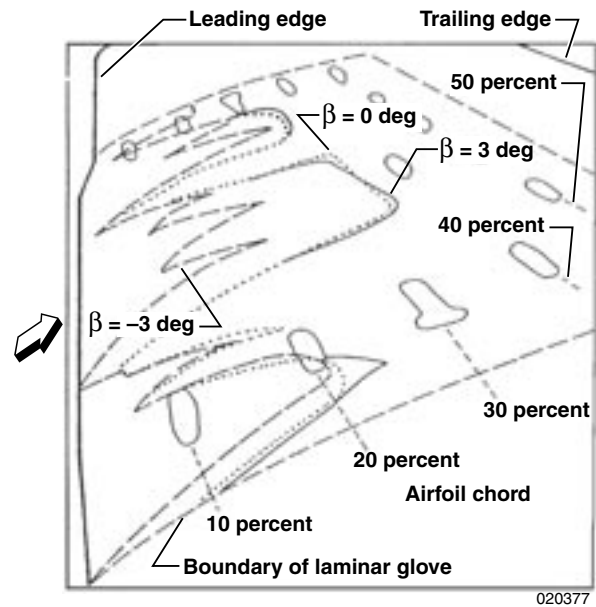
Figure 4.2.1-10. Drawing of transition lines on the VFW614/ATTAS glove for different yaw angles at flow conditions governed by crossflow instability.
