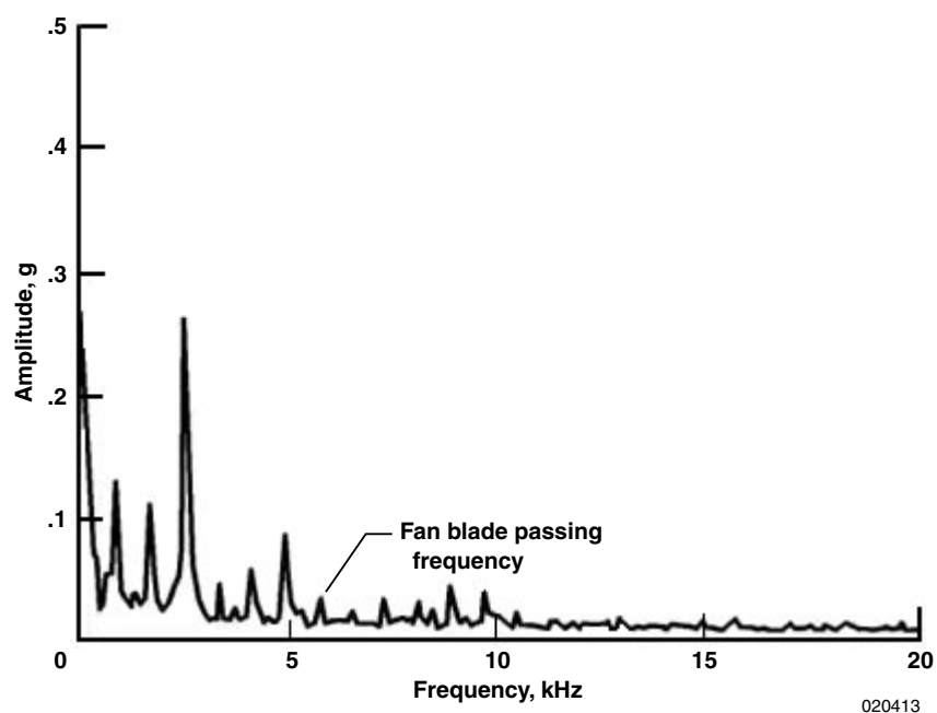
Figure 4.4-1. Vibration amplitudes as function of frequency measured by the accelerometers on the ATTAS NLF nacelle fan cowl at maximum cruise condition.
