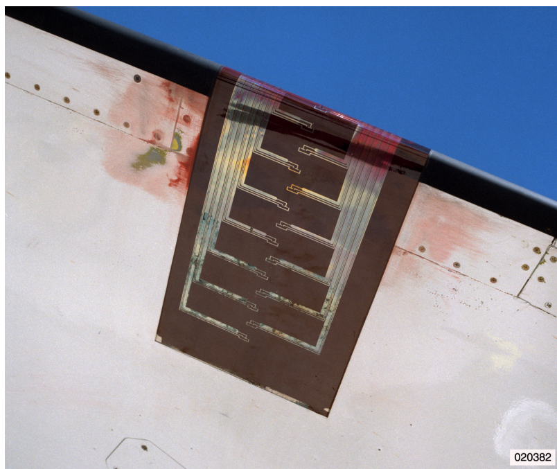
(a) Hot-film sensor array.
