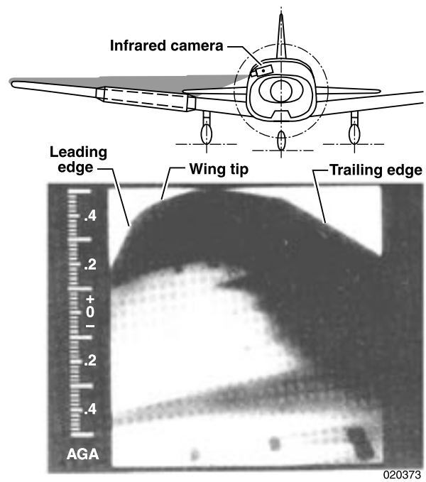
Figure 4.2.1-5. Infrared image of the LFU 205 glove in free flight, inverted image; laminar boundary layer white, turbulent dark.
