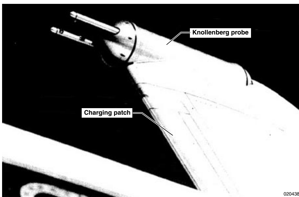
Figure 4.6-1. Cloud particle detection on JetStar pylon.
