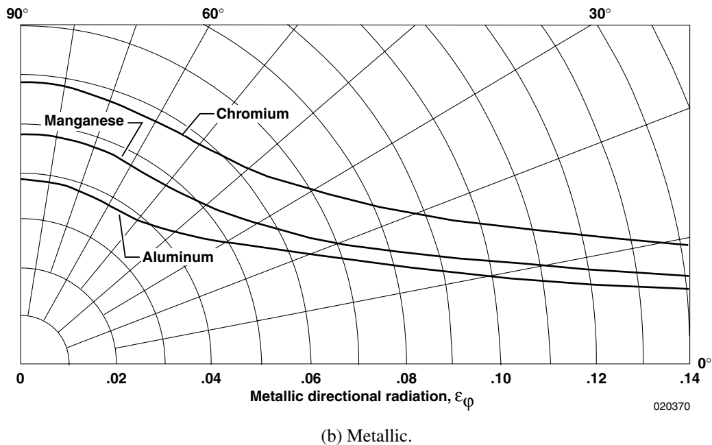
Figure 4.2.1-2. Directional radiation properties of nonmetallic and metallic surfaces.
