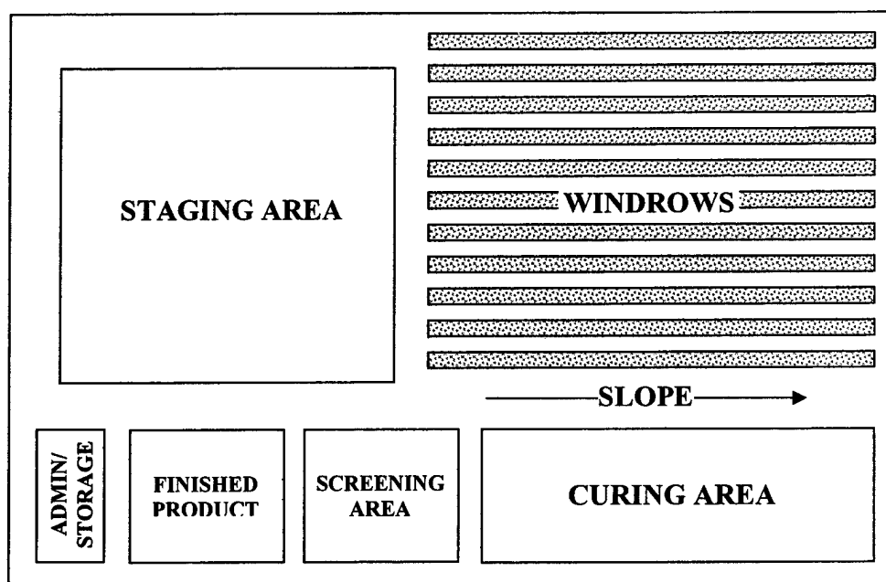
Figure 12.6 Typical Site Layout for a Compost Facility
