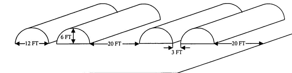
Figures 12.4 Low Technology Configuration of Windrows on Compost Pad
