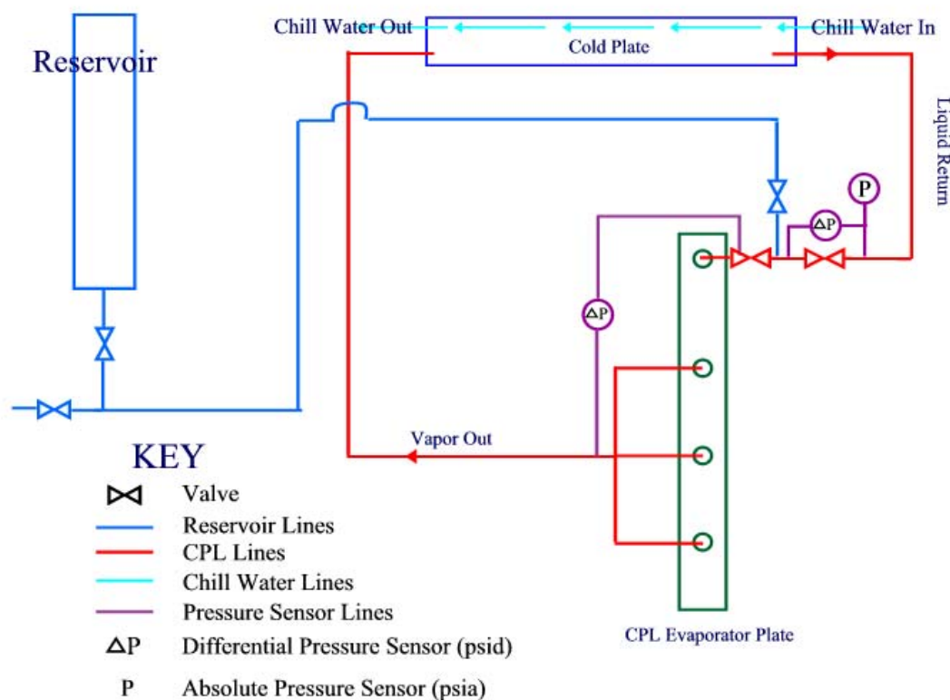
Figure 45: Loop Schematic
