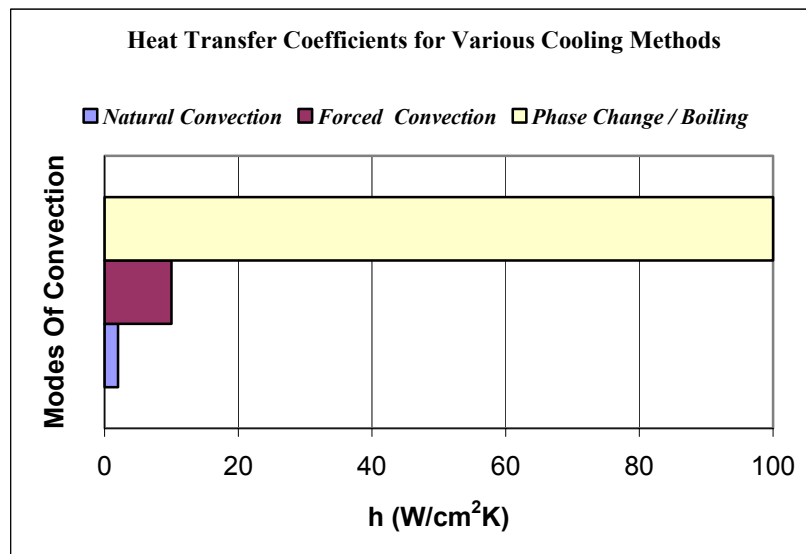
Figure 4: Cooling potentials for various cooling techniques (Kuszeowski 2002)
