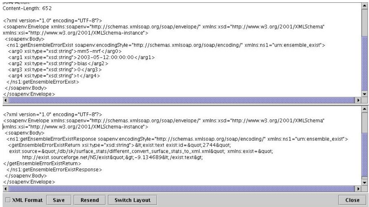
Figure 11. tcpmon GUI Showing Communication Between a Client, Requesting Statistics from an XML Database, and the Server Response.
