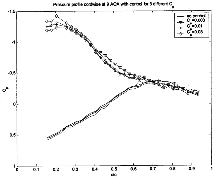
Figure 19: Averaged pressure distributions over the suction and the pressure side of the airfoil for \alpha=9^\circ .
