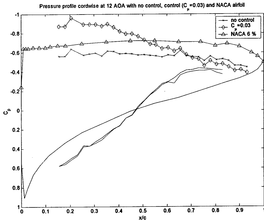
Figure 26: Comparison of present data, controlled and uncontrolled, with the data of Ref. 26, for \alpha=12^{\circ} .
