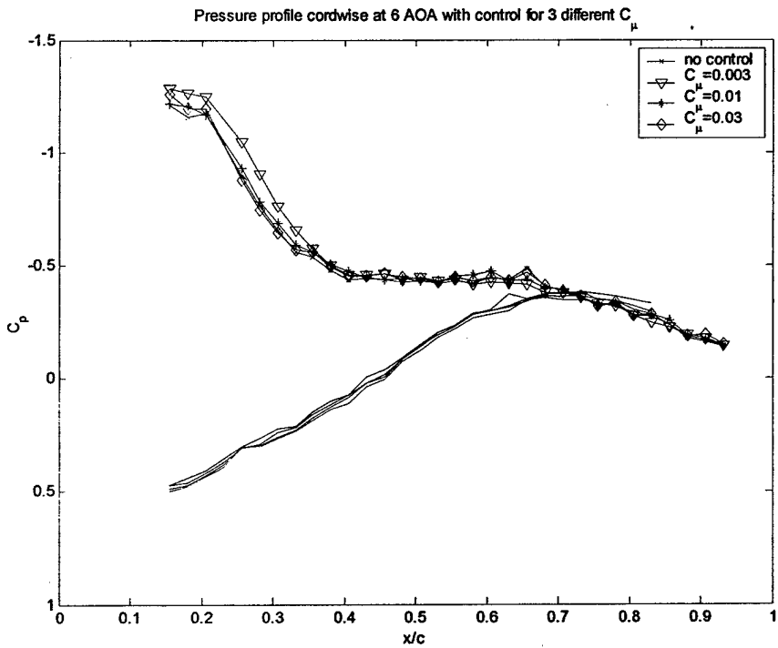
Figure 18: Averaged pressure distributions over the suction and the pressure side of the airfoil for \alpha=6^\circ
