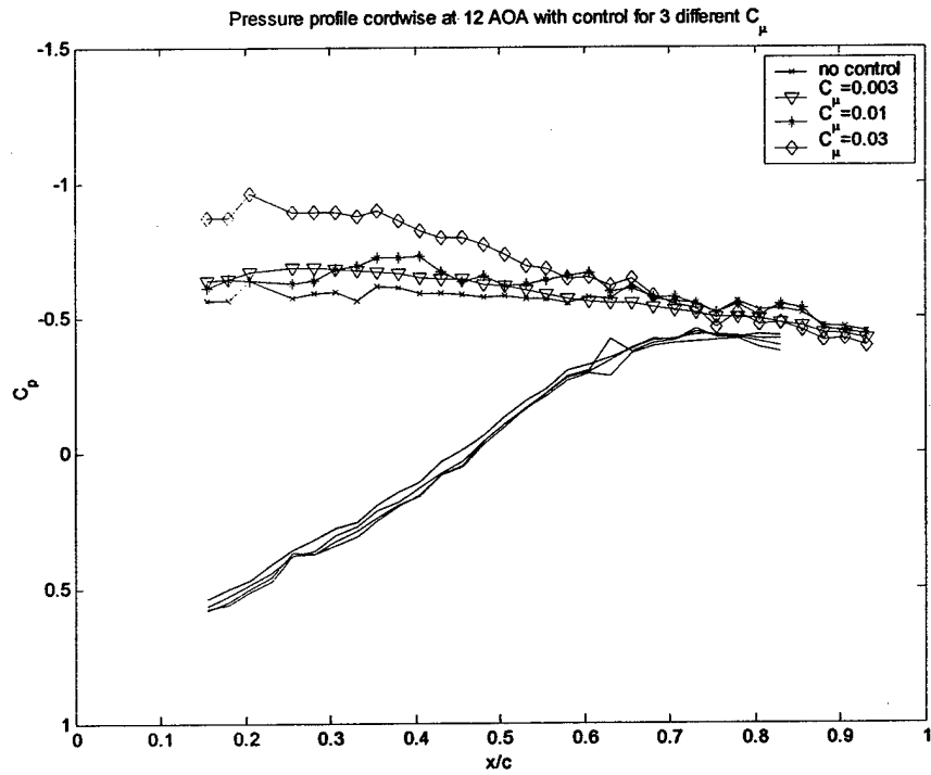
Figure 20: Averaged pressure distributions over the suction and the pressure side of the airfoil for \alpha=12^\circ .
