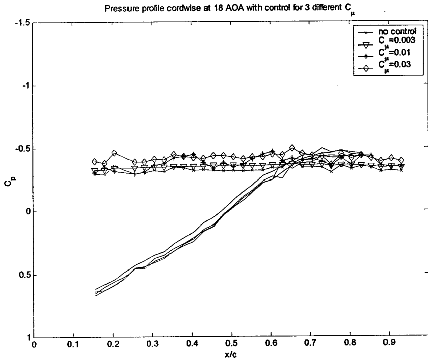
Figure 22: Averaged pressure distributions over the suction and the pressure side of the airfoil for \alpha=18^\circ .
