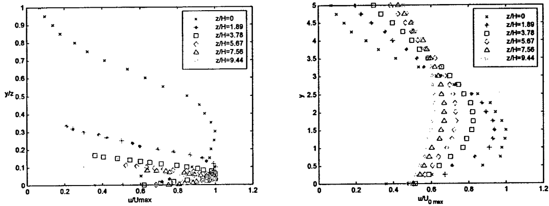
Figure 10: Actuator-jet velocity profiles in self-similar coordinates (left) and actual coordinates (right) 45 Hz
