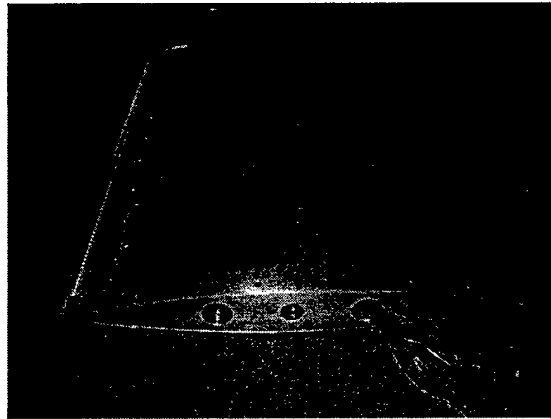
Figure 5: Photograph of the inside of the airfoil, showing the pneumatic flow control system and the pressure tubes. The skin of the model is open in this photograph. It bolts down on the bulkheads to form the shape of a sharp-edged airfoil.
