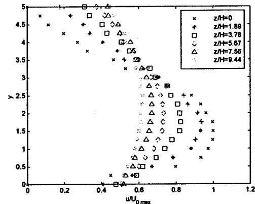
Figure 9: Actuator-jet velocity profiles in self-similar coordinates (left) and actual coordinates (right) 29 Hz
