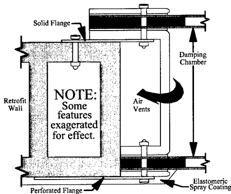
Figure 3. Flex-Retrofit Flange.
