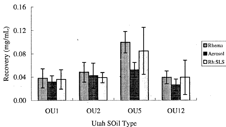
Figure 4.2: TCE Recovery for Batch Extraction Combined data sets, Methods 1 and 2
