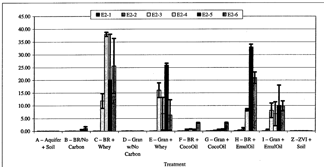
Figure 6.35. Variation of Fe 2+ over time in the complete culture augmentation study. Note bars represent 95% Confidence Intervals of the measurement.
