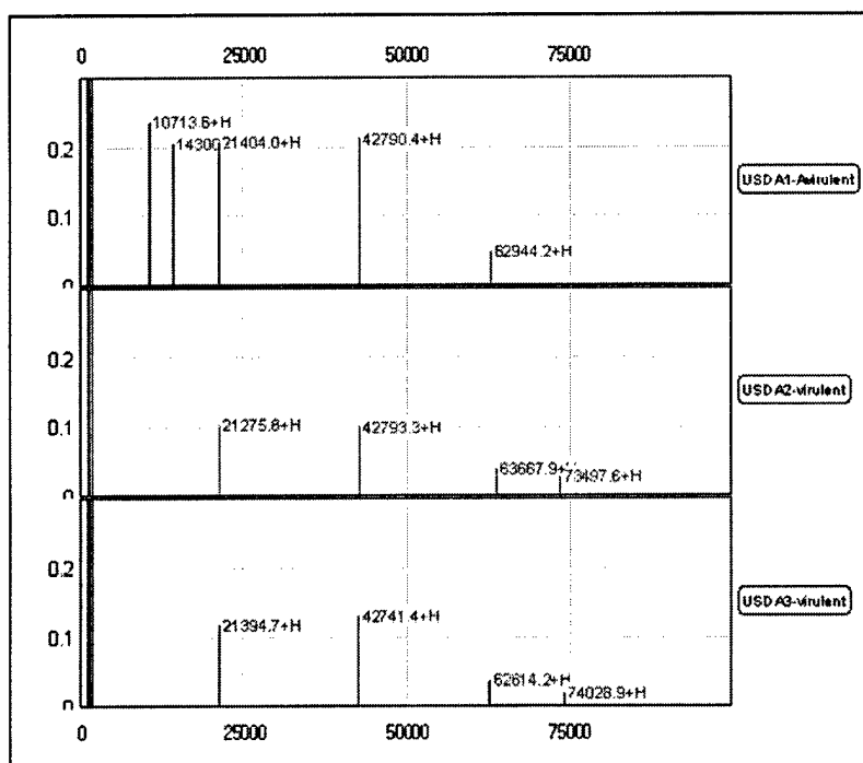
Figure 1. Mass spectrometry detection of extracellular products from virulent and avirulent strains of B. mallei grown in chemically defined media. Peaks of 10.7kD, 14.3kD can be seen from the sample obtained from the avirulent strain but absent in the 2 virulent strains examined. A peak at 74.5 kD was absent in the avirulent strain but present in both virulent strains
