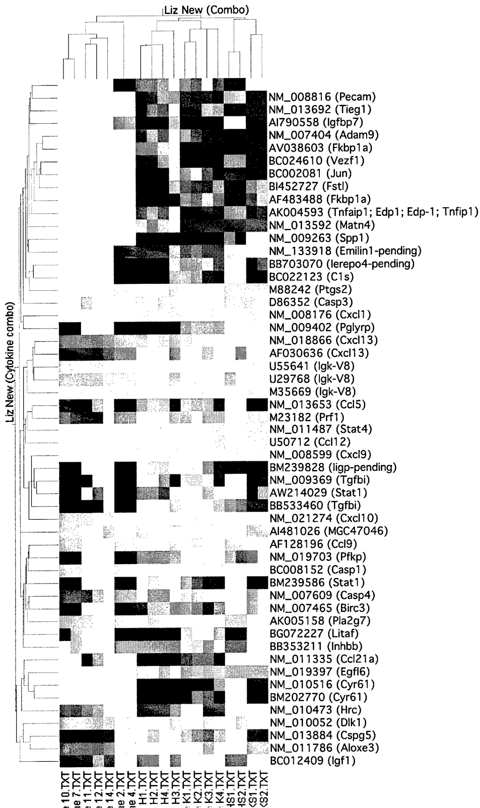
Selected Gene Tree: Liz New (Cytokine combo) Colored by: Liz New Selected Condition Tree: Liz New (Combo) Gene List: [Cytokine] and [Combo] (54)
