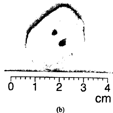
FIG. 4. Photoacoustic tomography of two slices of chicken gizzard that were buried 0.5 cm deep in the chicken breast slab. (a) Reconstructed image; (b) picture of the imaged cross-section of the sample.
