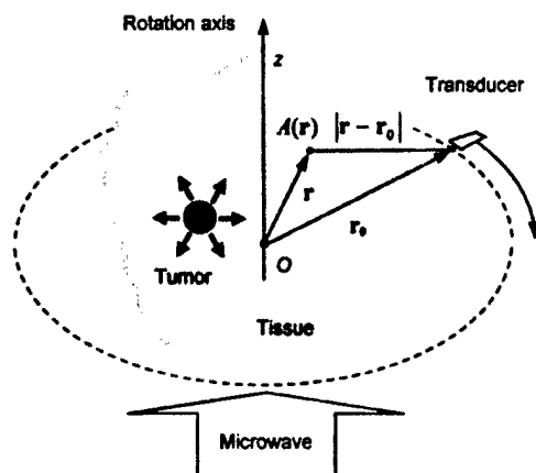
FIG. 1. Scheme of thermoacoustic circular measurement. Microwave pulses are transmitted to the sample from the bottom. The tumor inside absorbs the energy and generates thermoacoustic waves. An ultrasonic transducer at position r_0 records the thermoacoustic signals.
