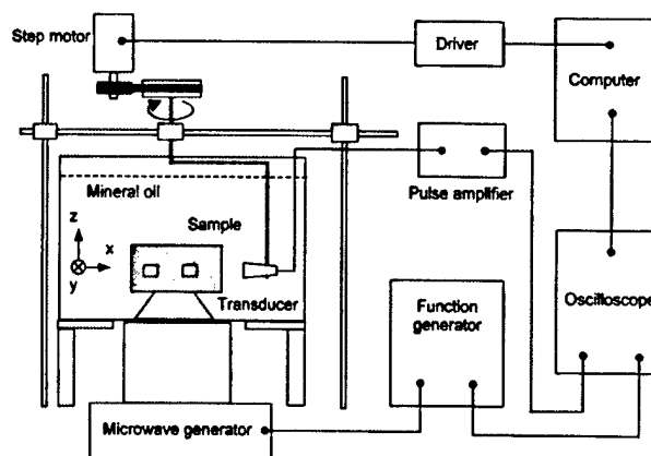
FIG. 2. Experimental setup.
